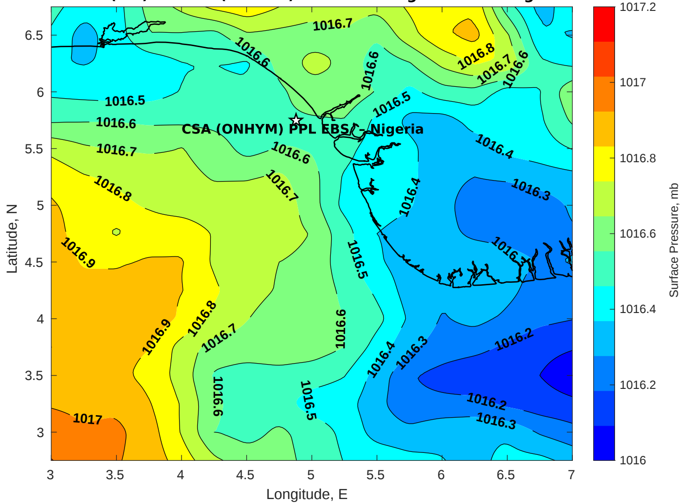
Surface Pressure (mb) for CSA (ONHYM) PPL EBS - Nigeria at 15-Aug-2025 00:00:00
