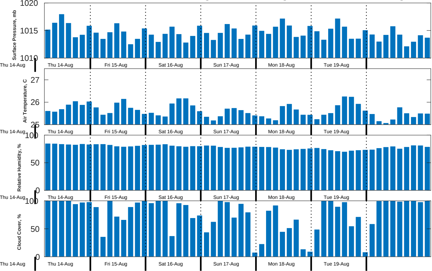
Met Forecast for CSA (ONHYM) PPL EBS - Nigeria from 15-Aug-2025 00:00:00 to 22-Aug-2025 00:00:00
