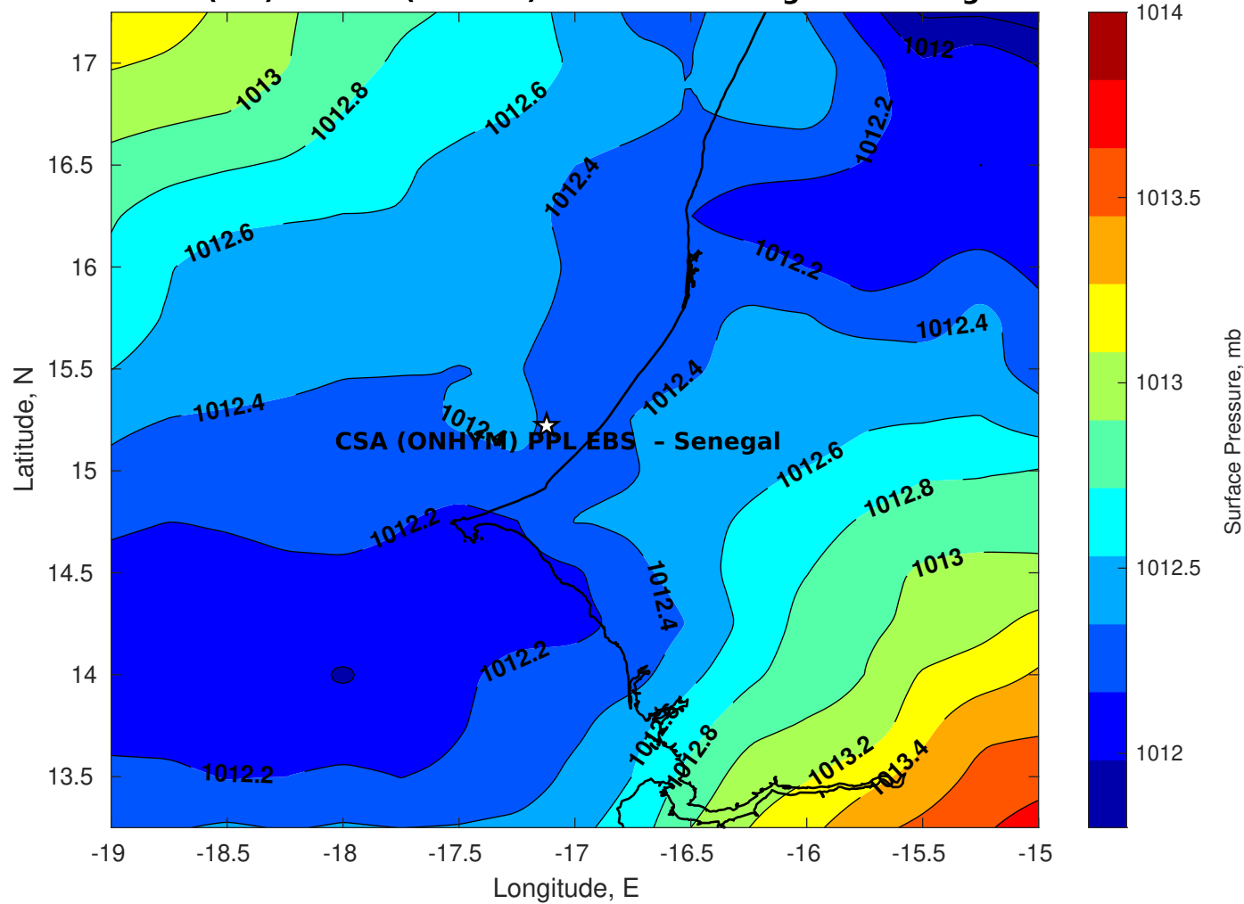
Surface Pressure (mb) for CSA (ONHYM) PPL EBS - Senegal at 17-Aug-2025 00:00:00
