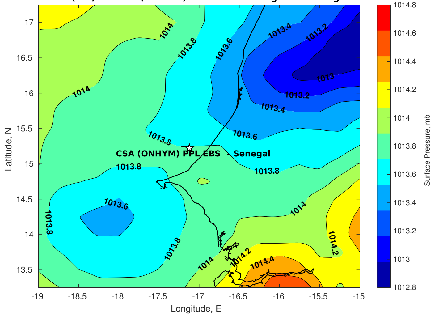
Surface Pressure (mb) for CSA (ONHYM) PPL EBS - Senegal at 16-Aug-2025 00:00:00
