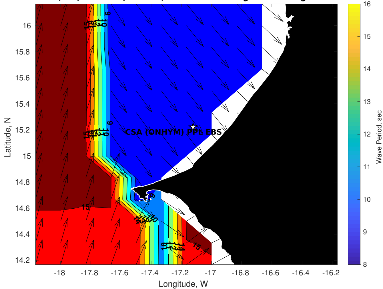
Wave Period (sec) for CSA (ONHYM) PPL EBS - Senegal at 15-Aug-2025 09:00:00
