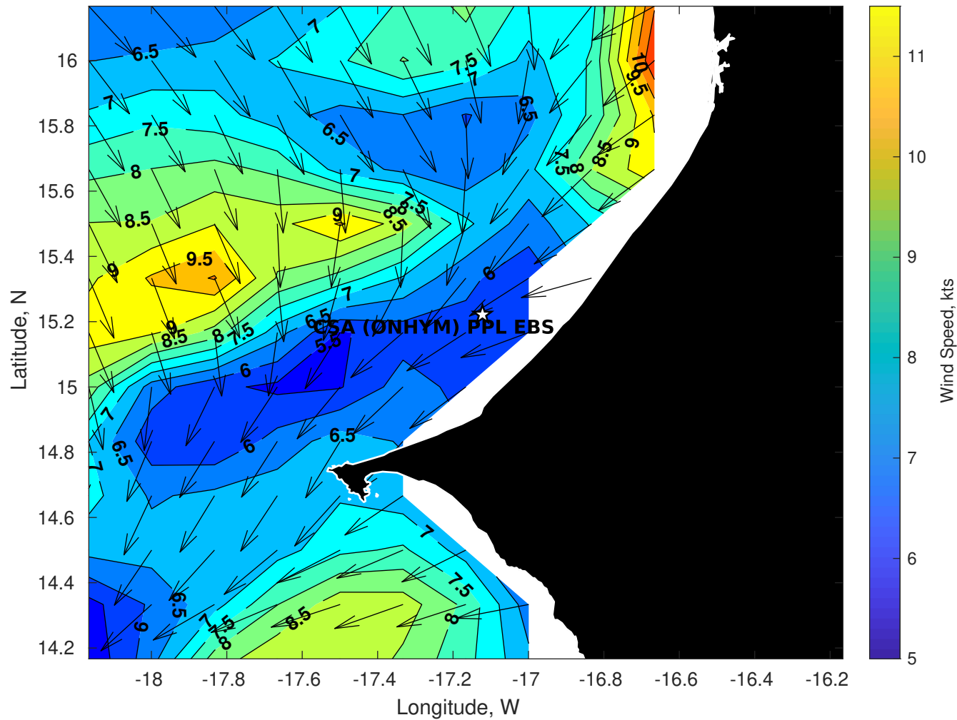
Winds (kts) for CSA (ONHYM) PPL EBS - Senegal at 15-Aug-2025 09:00:00
