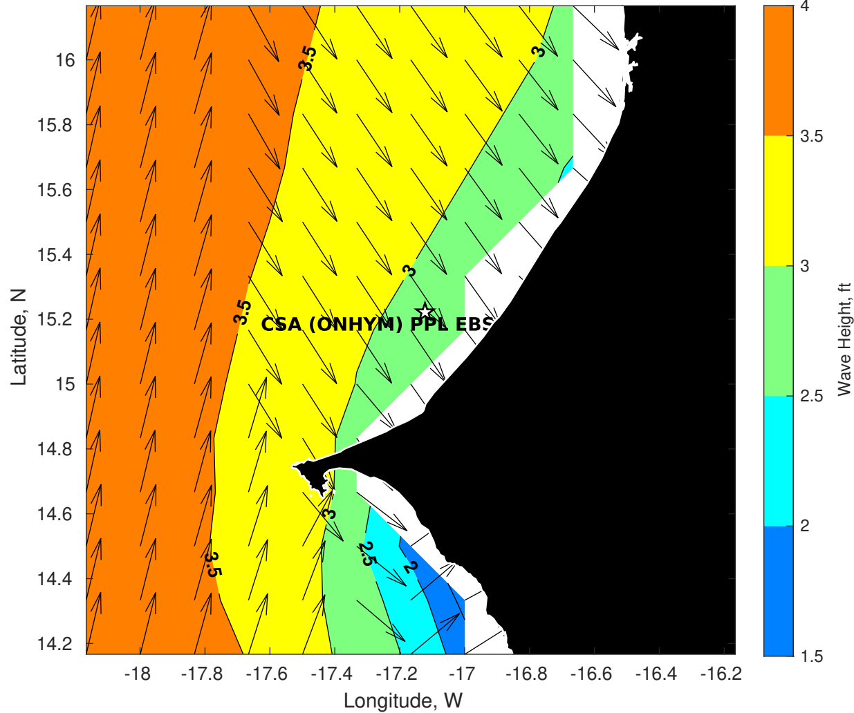
Wave Height (ft) for CSA (ONHYM) PPL EBS - Senegal at 15-Aug-2025 09:00:00
