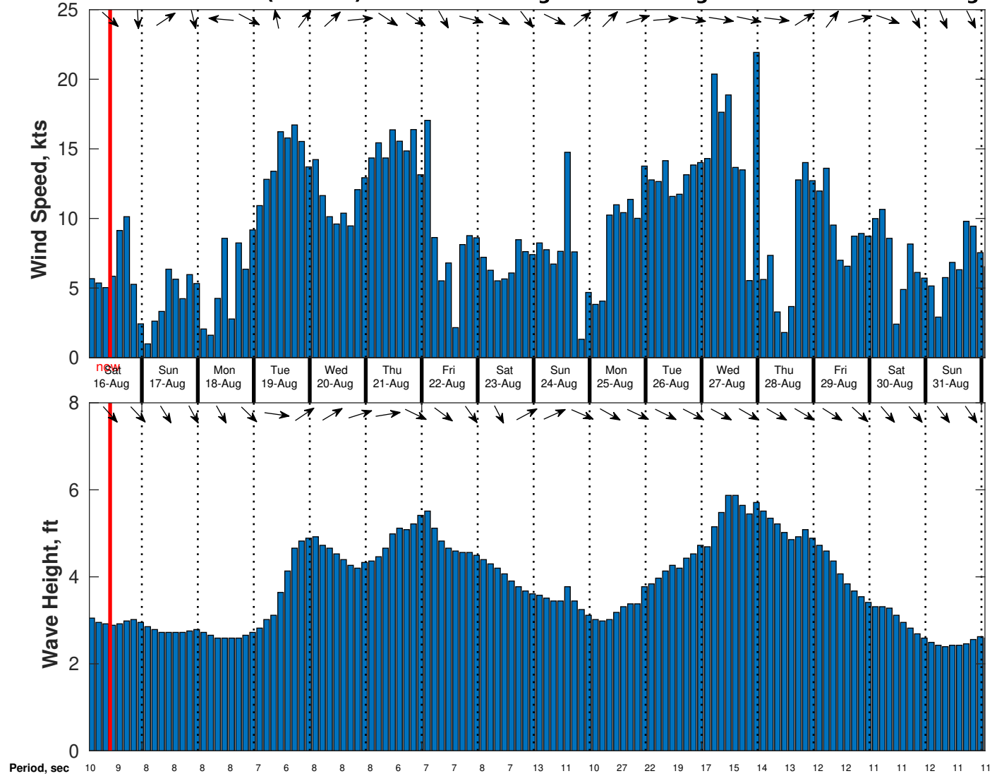
Wind & Wave Forecast for CSA (ONHYM) PPL EBS - Senegal from 15-Aug-2025 01:00:00 to 31-Aug-2025 01:00:00
