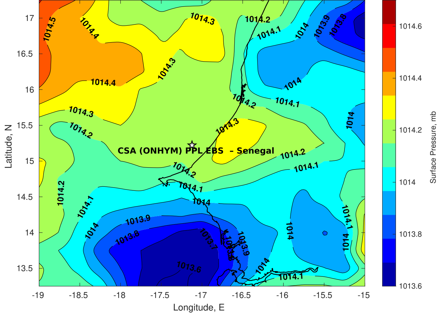
Surface Pressure (mb) for CSA (ONHYM) PPL EBS - Senegal at 15-Aug-2025 00:00:00
