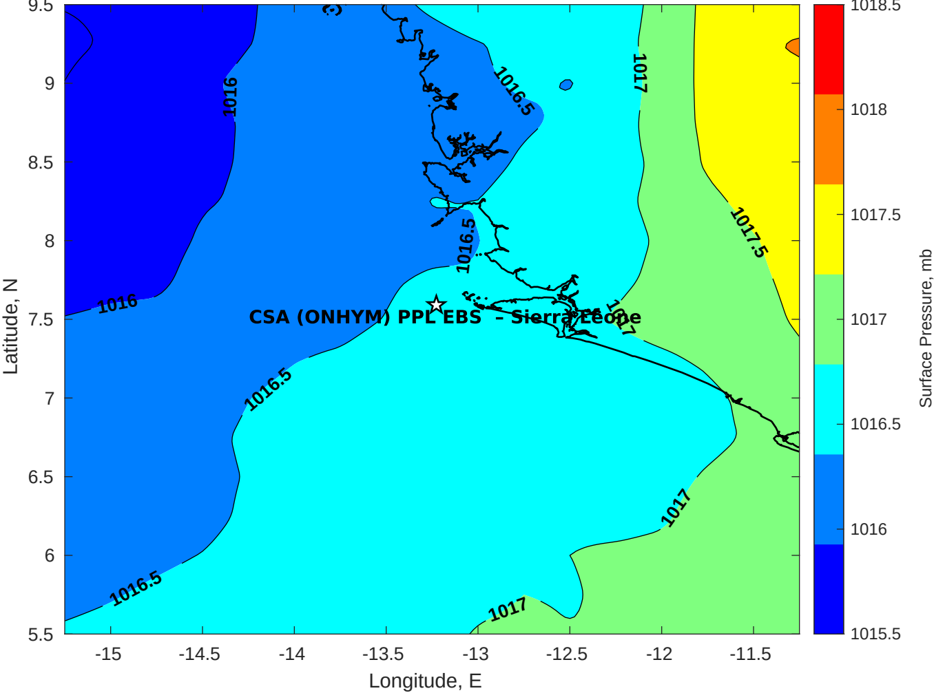
Surface Pressure (mb) for CSA (ONHYM) PPL EBS - Sierra Leone at 15-Aug-2025 00:00:00
