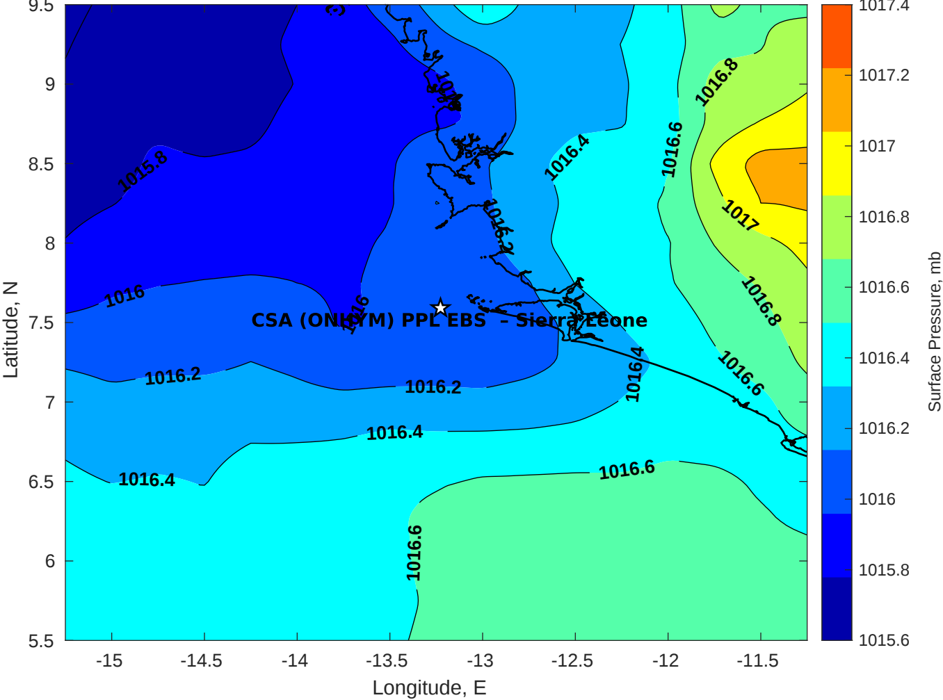
Surface Pressure (mb) for CSA (ONHYM) PPL EBS - Sierra Leone at 16-Aug-2025 00:00:00
