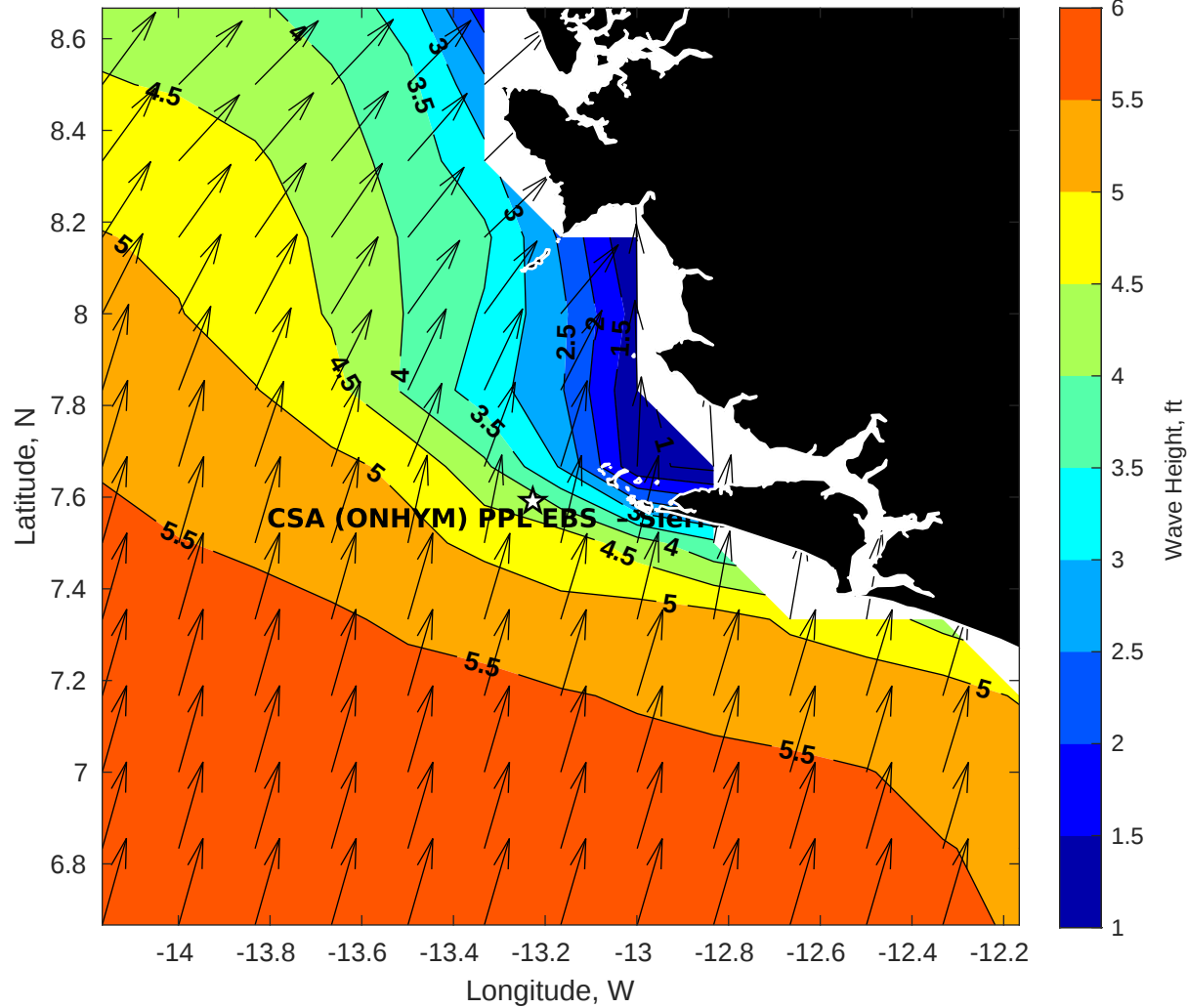
Wave Height (ft) for CSA (ONHYM) PPL EBS - Sierra Leone at 15-Aug-2025 09:00:00
