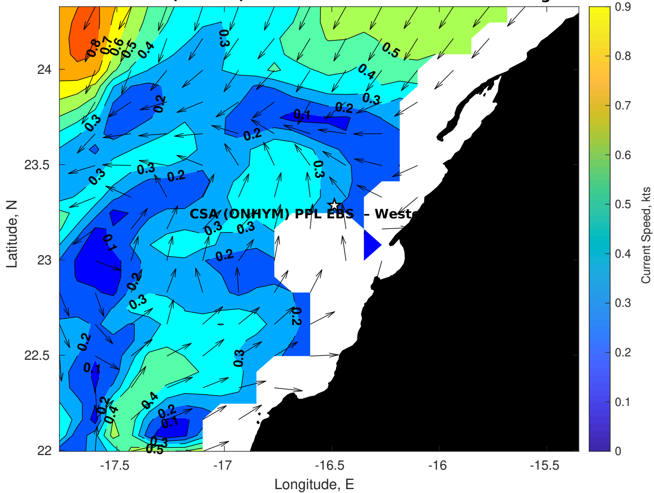
Surface Currents for CSA (ONHYM) PPL EBS - Western Sahara at 14-Aug-2025 00:00:00
