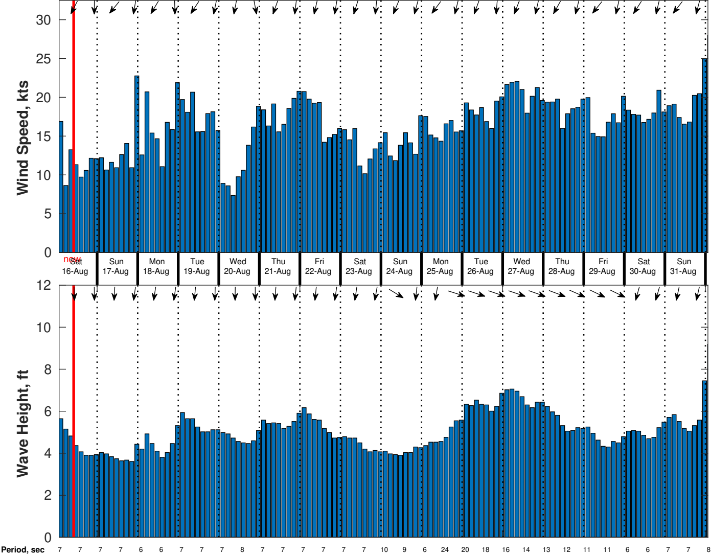
Wind & Wave Forecast for CSA (ONHYM) PPL EBS - Western Sahara from 15-Aug-2025 01:00:00 to 31-Aug-2025 01:00:00
