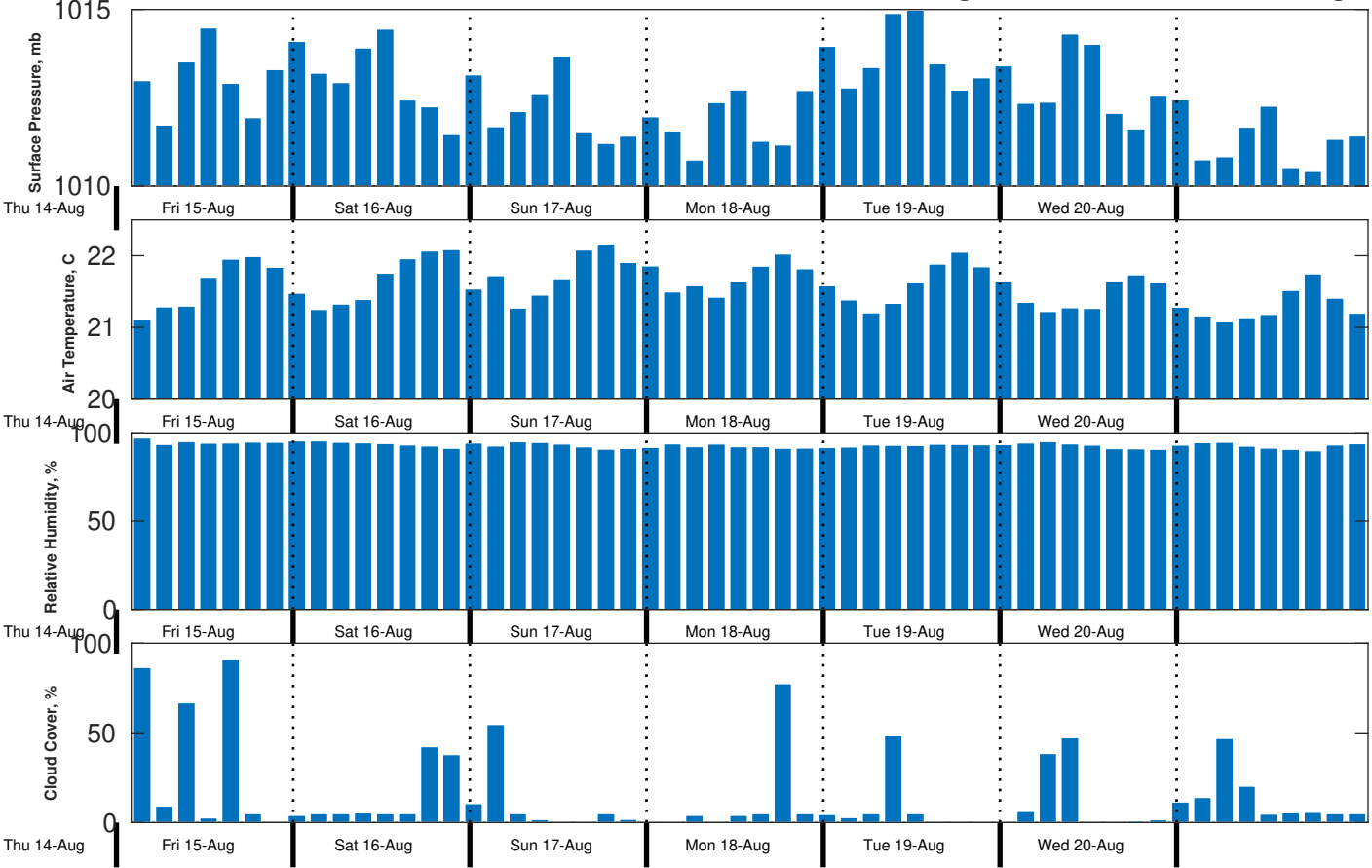
Met Forecast for CSA (ONHYM) PPL EBS - Western Sahara from 15-Aug-2025 00:00:00 to 22-Aug-2025 00:00:00
