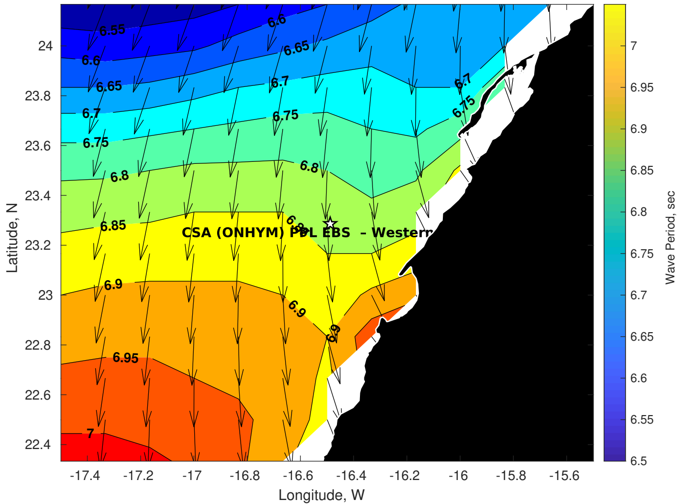
Wave Period (sec) for CSA (ONHYM) PPL EBS - Western Sahara at 15-Aug-2025 09:00:00
