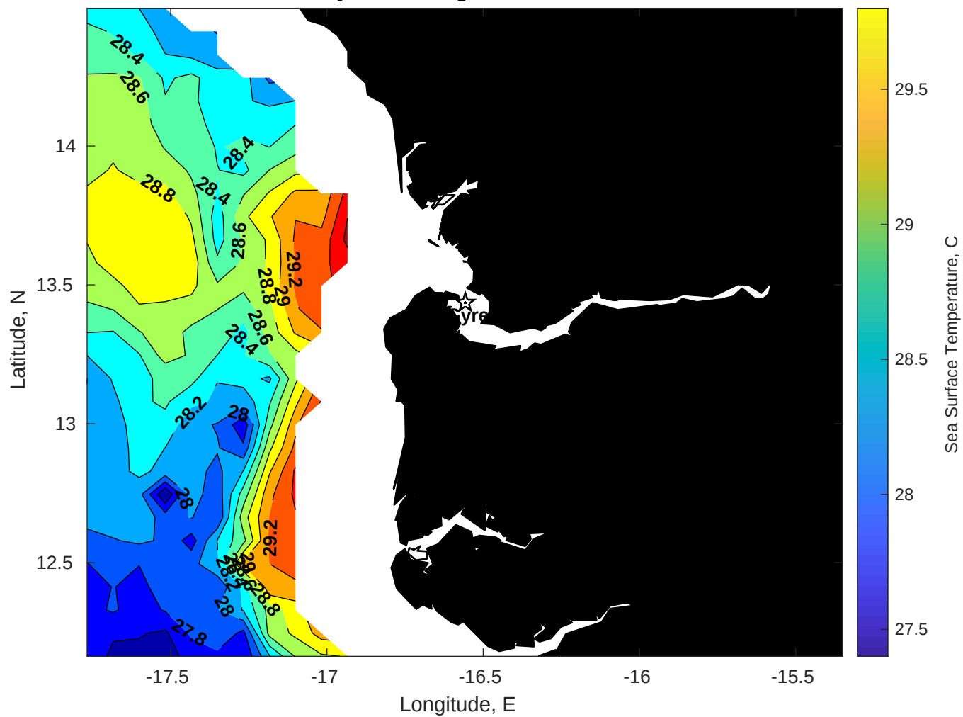
SST for Gyre at 14-Aug-2025 00:00:00
