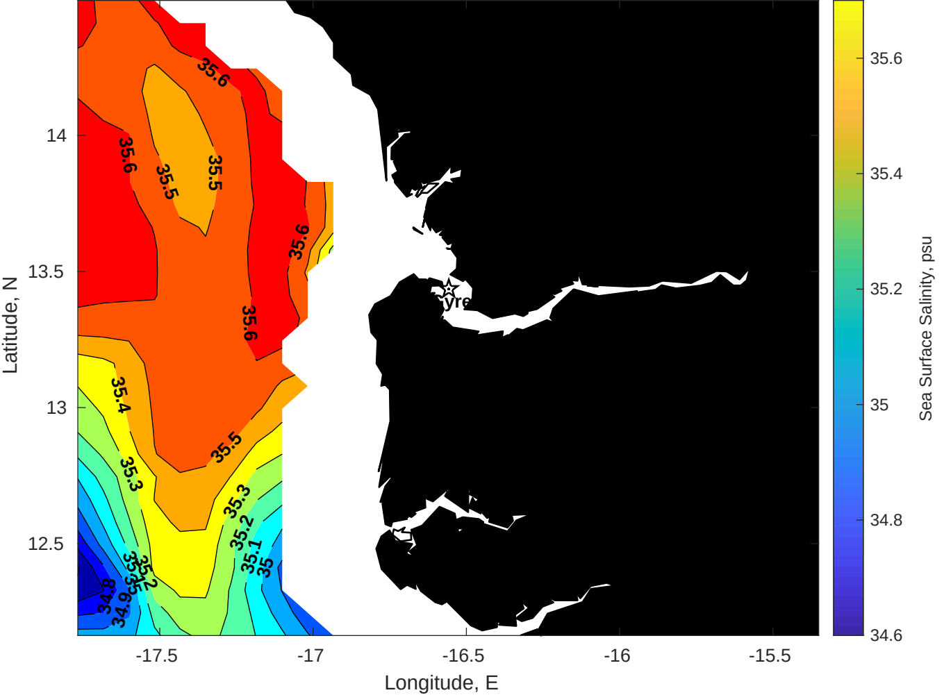
Surface Salinity for Gyre at 14-Aug-2025 00:00:00
