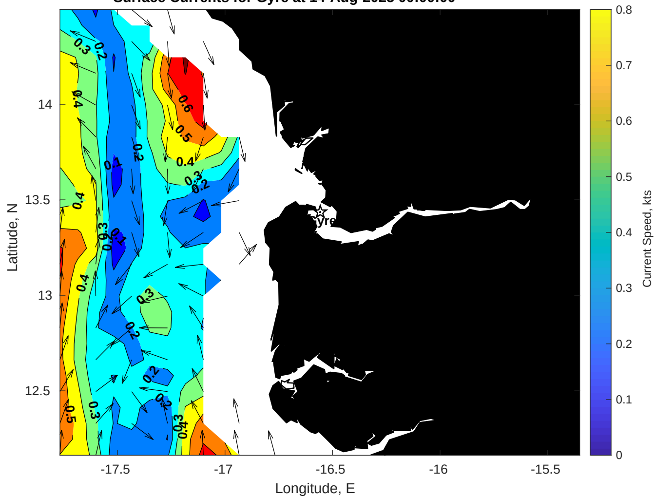
Surface Currents for Gyre at 14-Aug-2025 00:00:00
