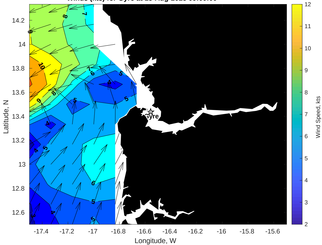
Winds (kts) for Gyre at 15-Aug-2025 09:00:00
