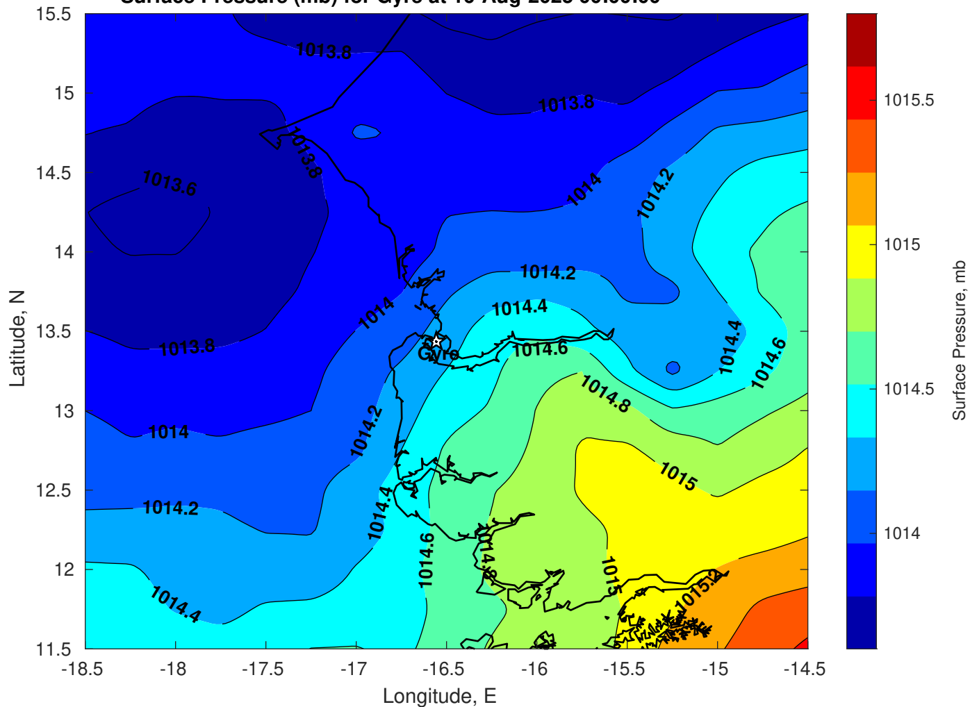
Surface Pressure (mb) for Gyre at 16-Aug-2025 00:00:00
