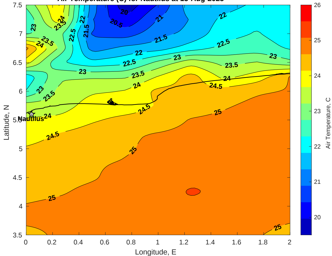
Air Temperature (C) for Nautilus at 15-Aug-2025
