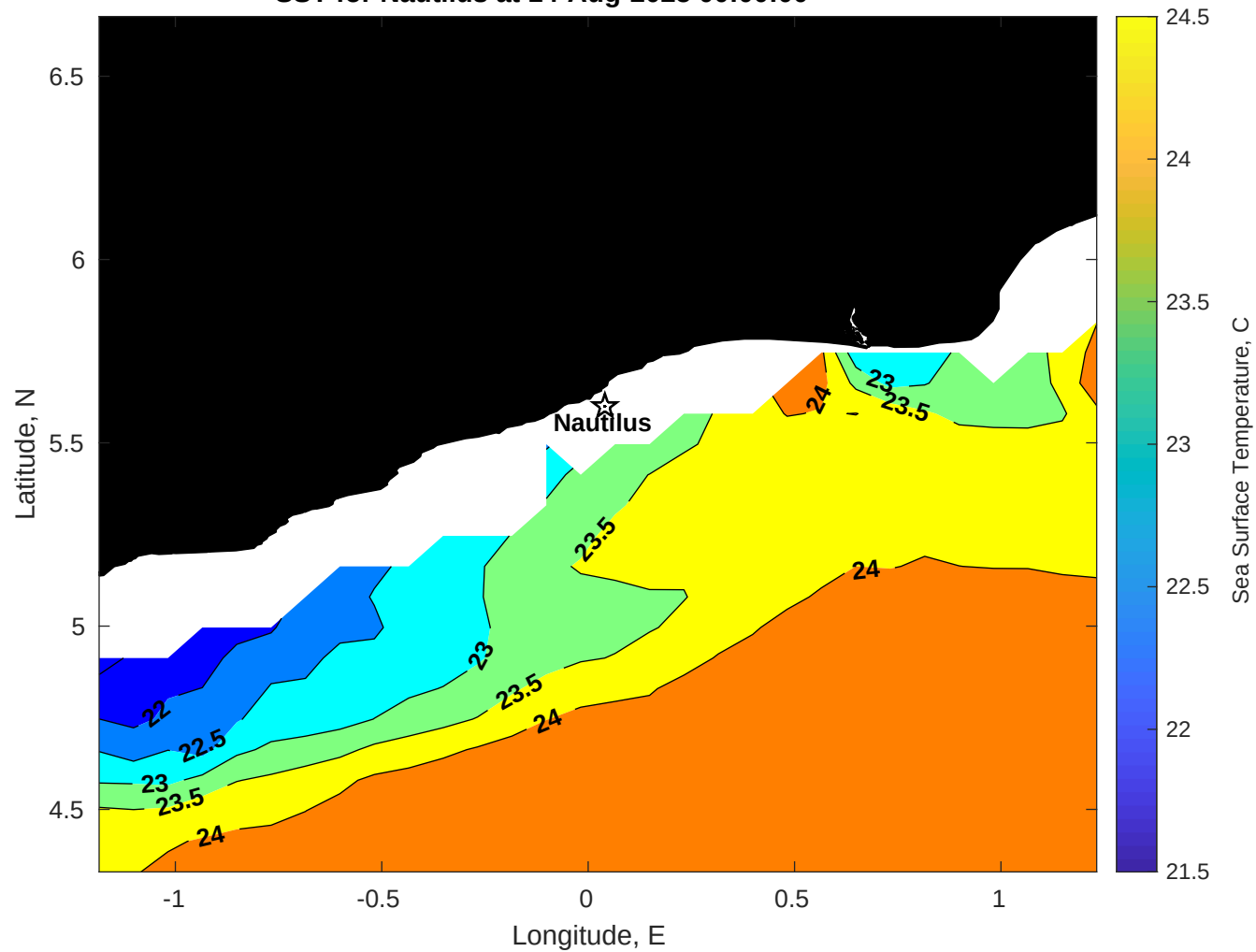
SST for Nautilus at 14-Aug-2025 00:00:00
