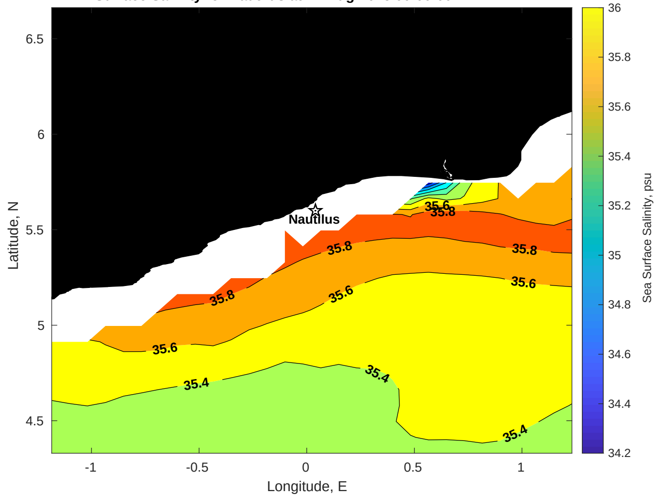
Surface Salinity for Nautilus at 14-Aug-2025 00:00:00
