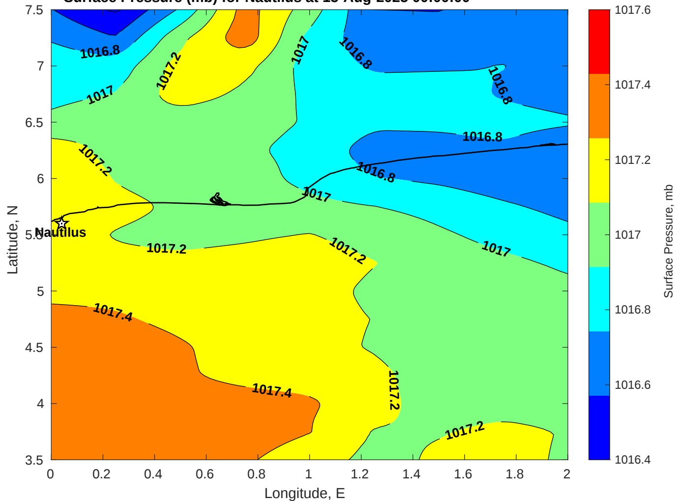
Surface Pressure (mb) for Nautilus at 15-Aug-2025 00:00:00
