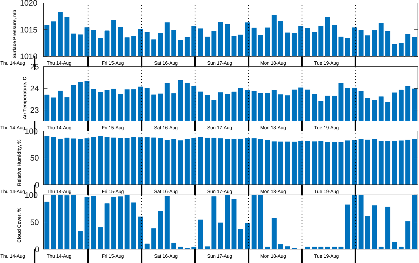
Met Forecast for Nautilus from 15-Aug-2025 00:00:00 to 22-Aug-2025 00:00:00
