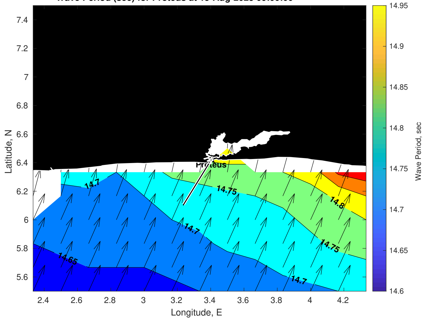
Wave Period (sec) for Proteus at 15-Aug-2025 09:00:00
