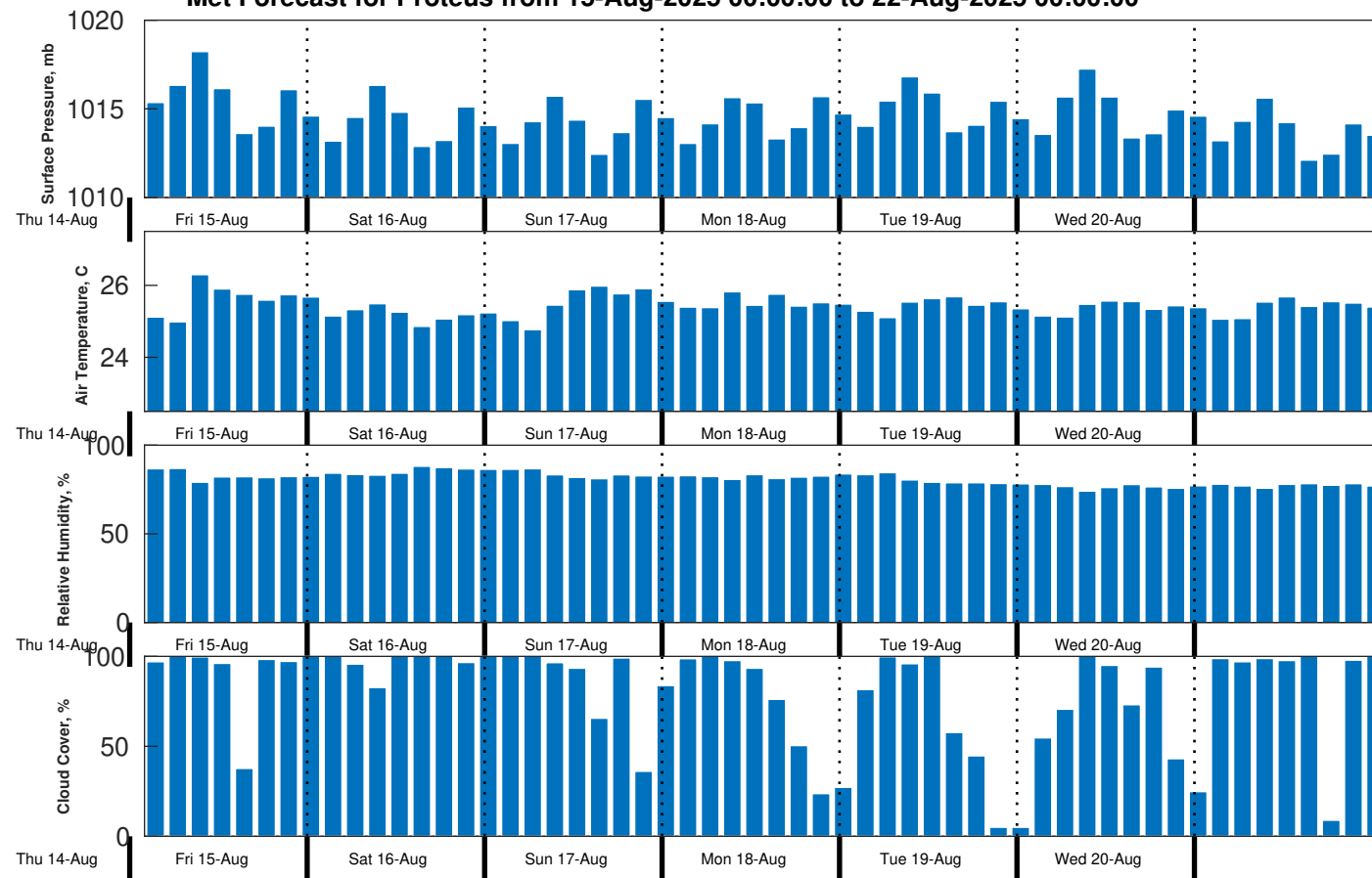
Met Forecast for Proteus from 15-Aug-2025 00:00:00 to 22-Aug-2025 00:00:00
