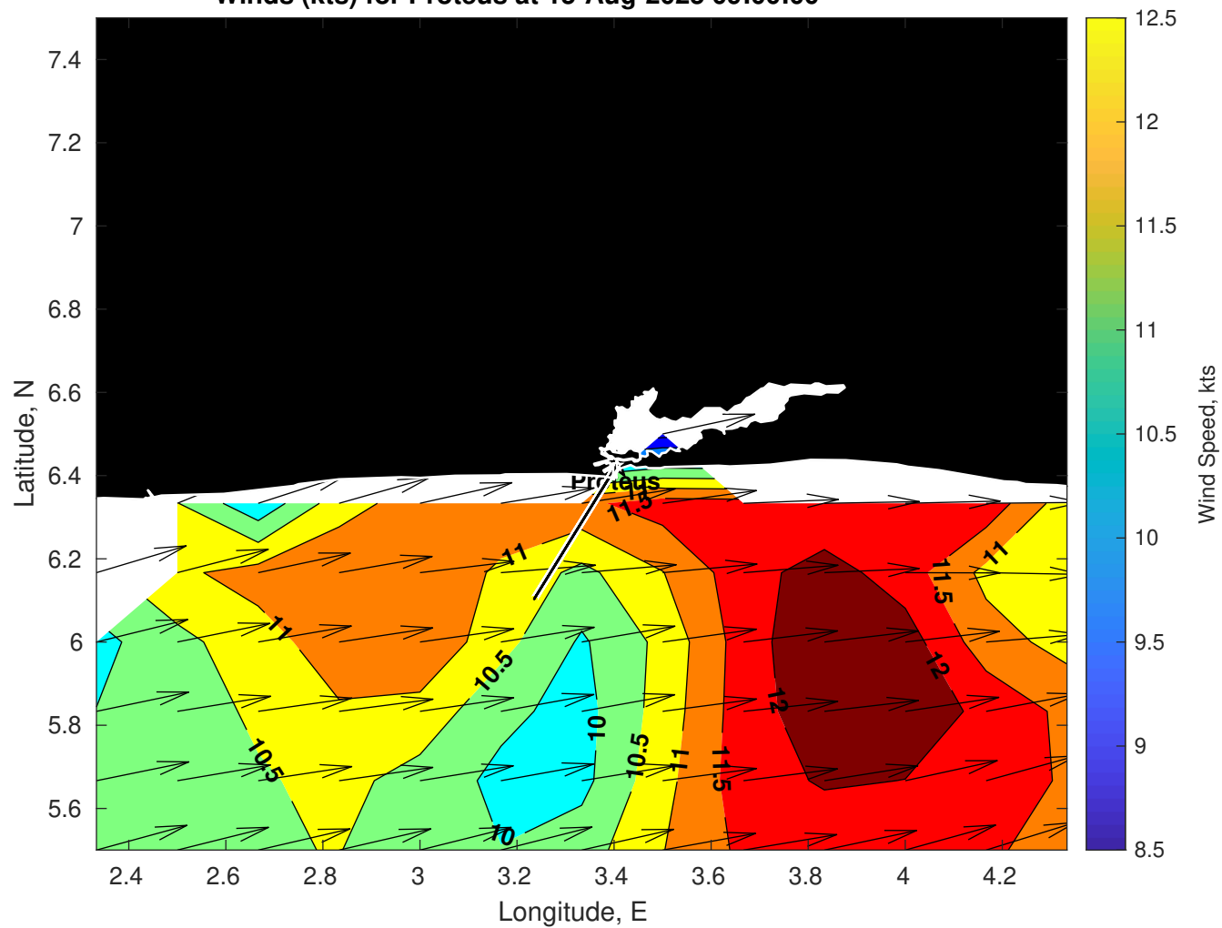
Winds (kts) for Proteus at 15-Aug-2025 09:00:00
