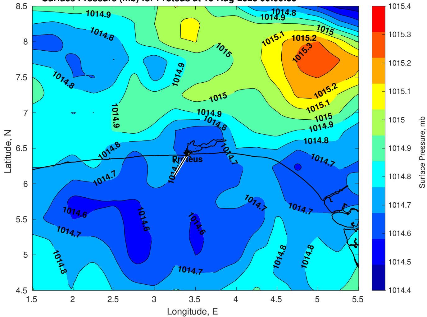
Surface Pressure (mb) for Proteus at 16-Aug-2025 00:00:00
