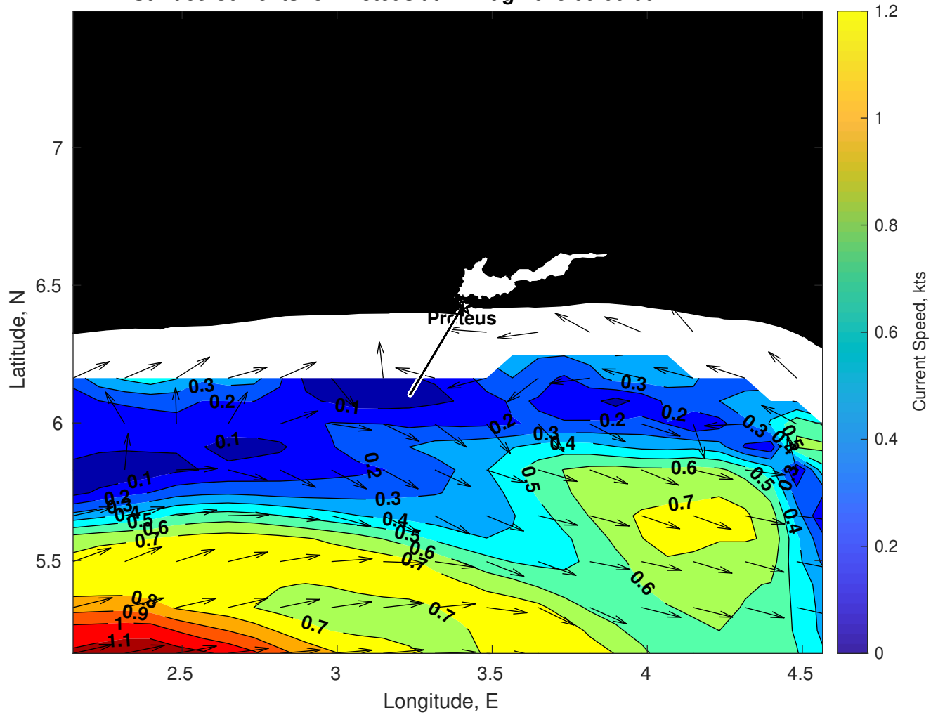
Surface Currents for Proteus at 14-Aug-2025 00:00:00
