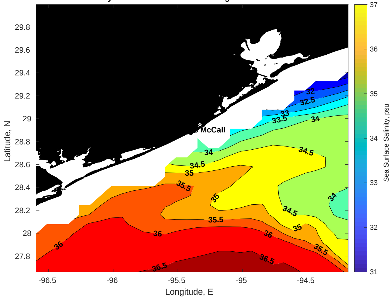
Surface Salinity for Brooks McCall at 15-Aug-2025 00:00:00
