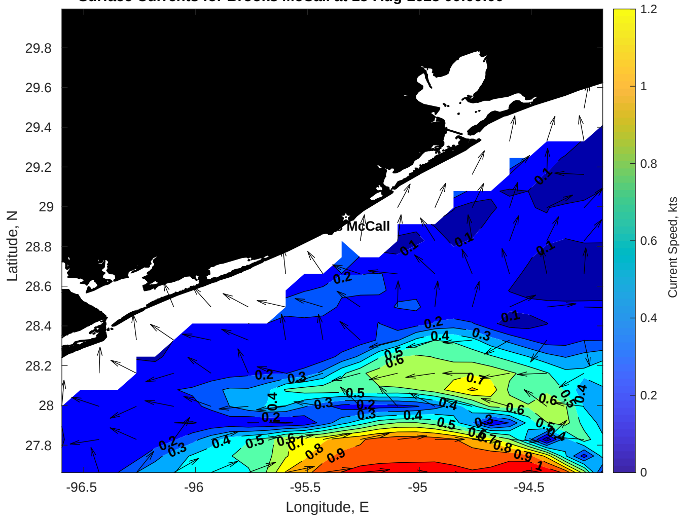
Surface Currents for Brooks McCall at 15-Aug-2025 00:00:00
