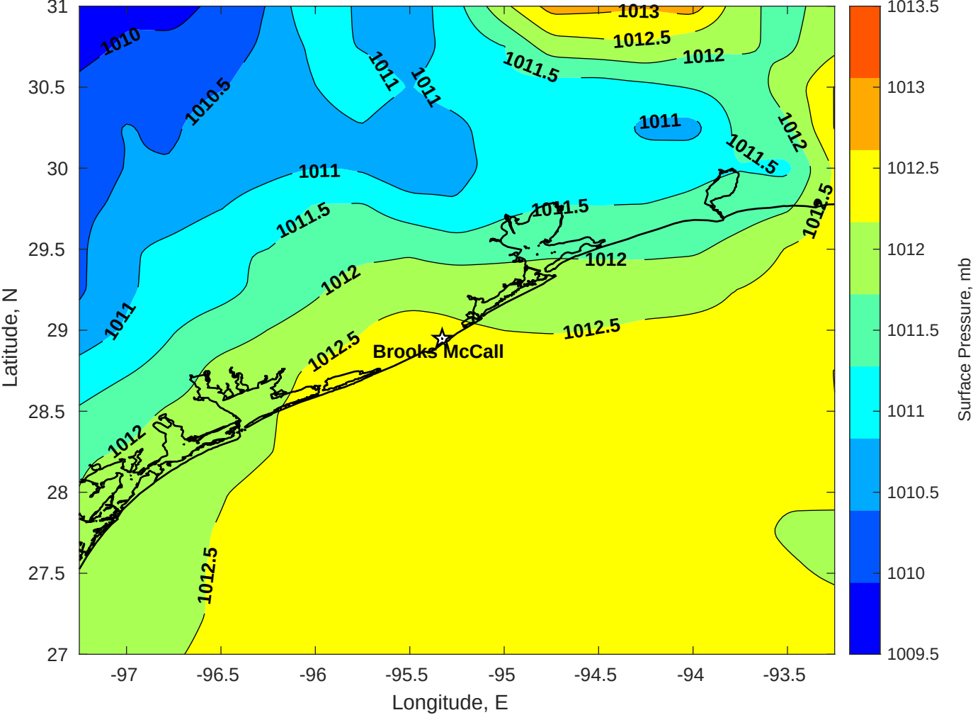
Surface Pressure (mb) for Brooks McCall at 18-Aug-2025 00:00:00
