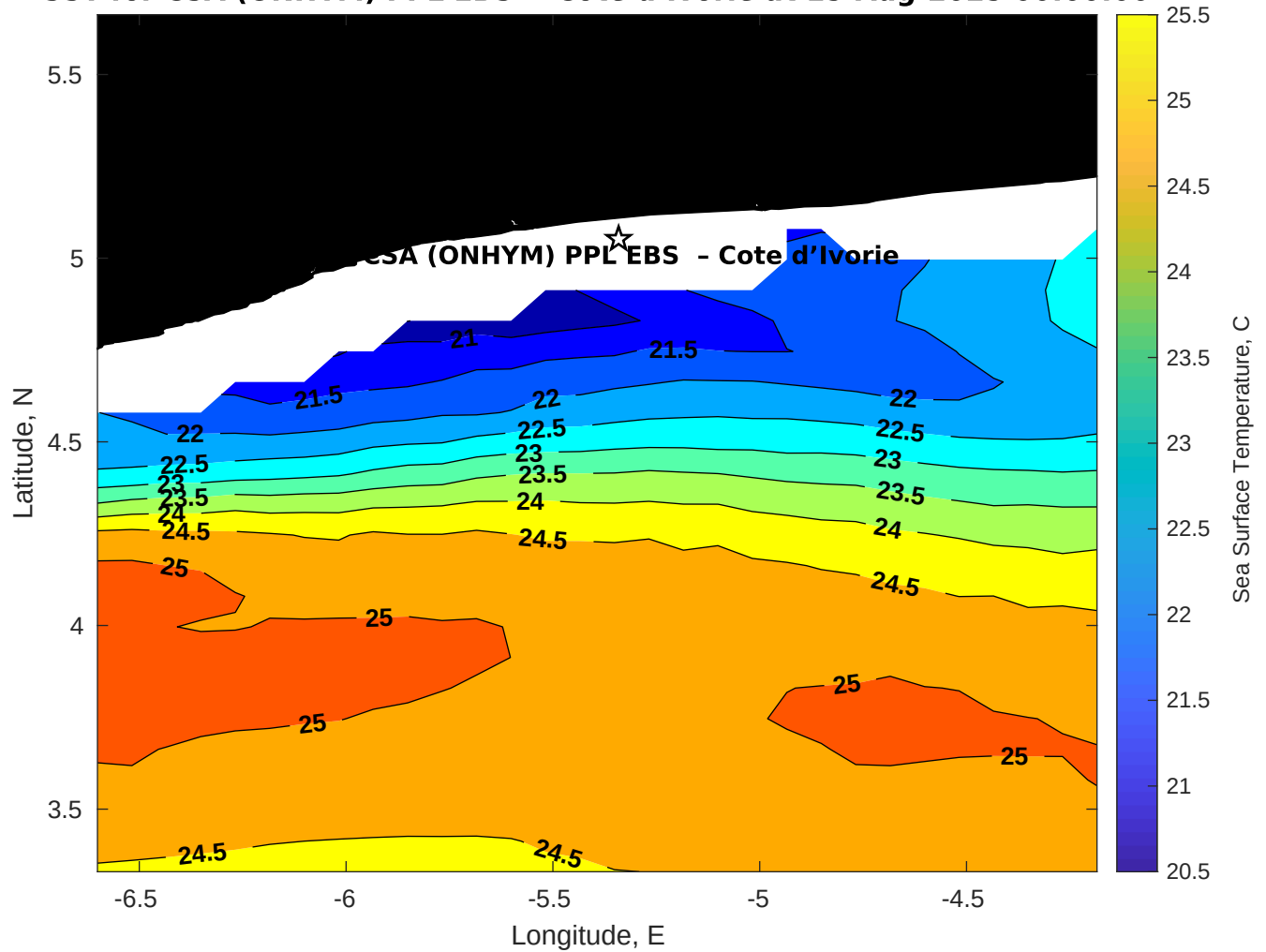
SST for CSA (ONHYM) PPL EBS - Cote d'Ivoire at 15-Aug-2025 00:00:00
