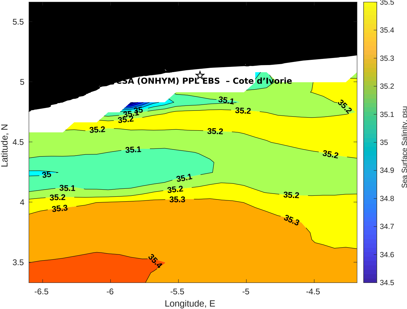
Surface Salinity for CSA (ONHYM) PPL EBS - Cote d'Ivoire at 15-Aug-2025 00:00:00
