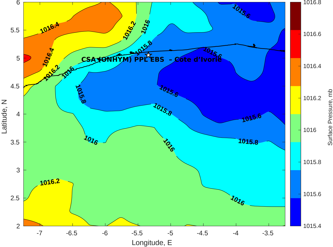
Surface Pressure (mb) for CSA (ONHYM) PPL EBS - Cote d'Ivoire at 16-Aug-2025 00:00:00
