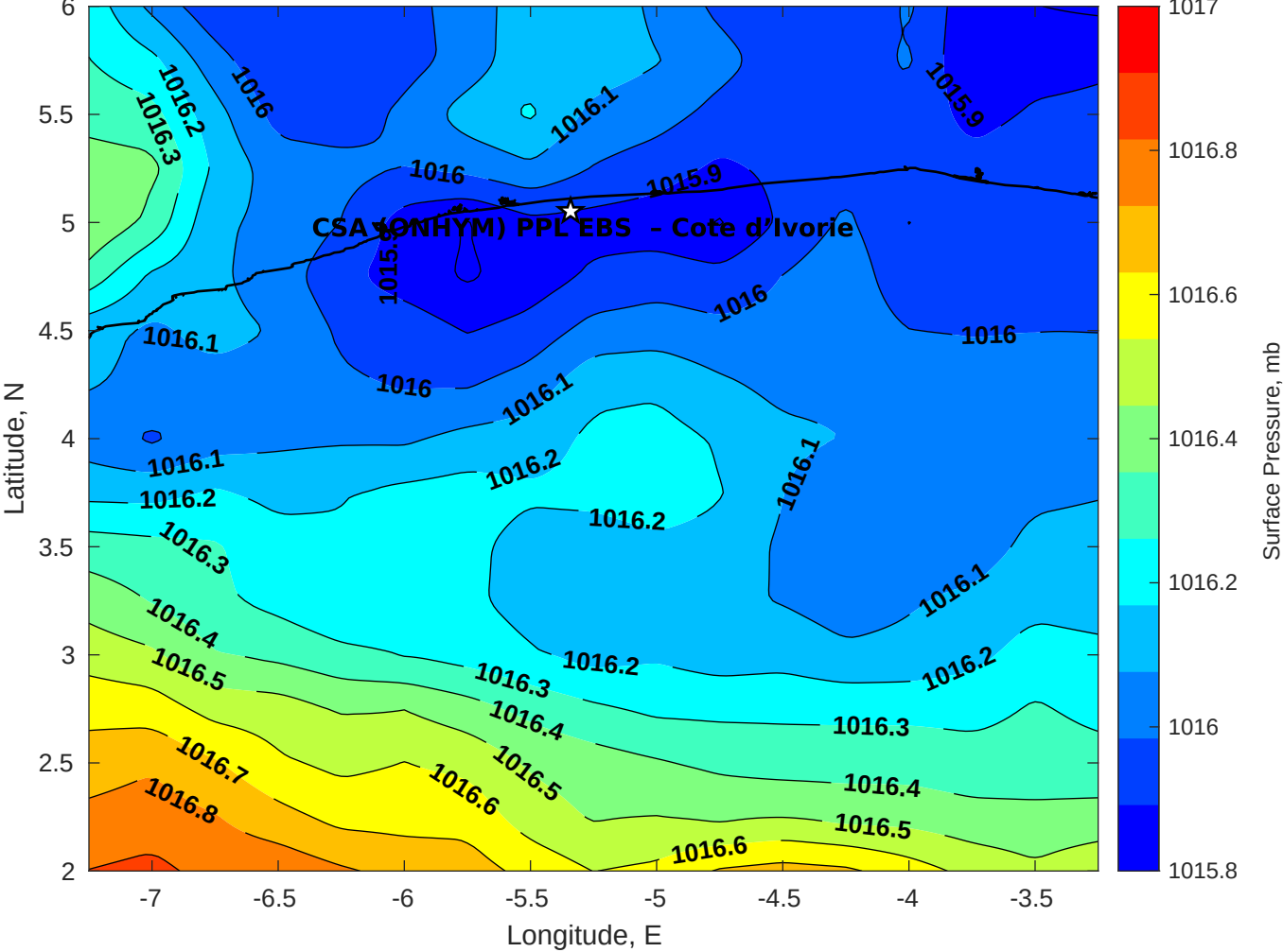
Surface Pressure (mb) for CSA (ONHYM) PPL EBS - Cote d'Ivoire at 18-Aug-2025 00:00:00
