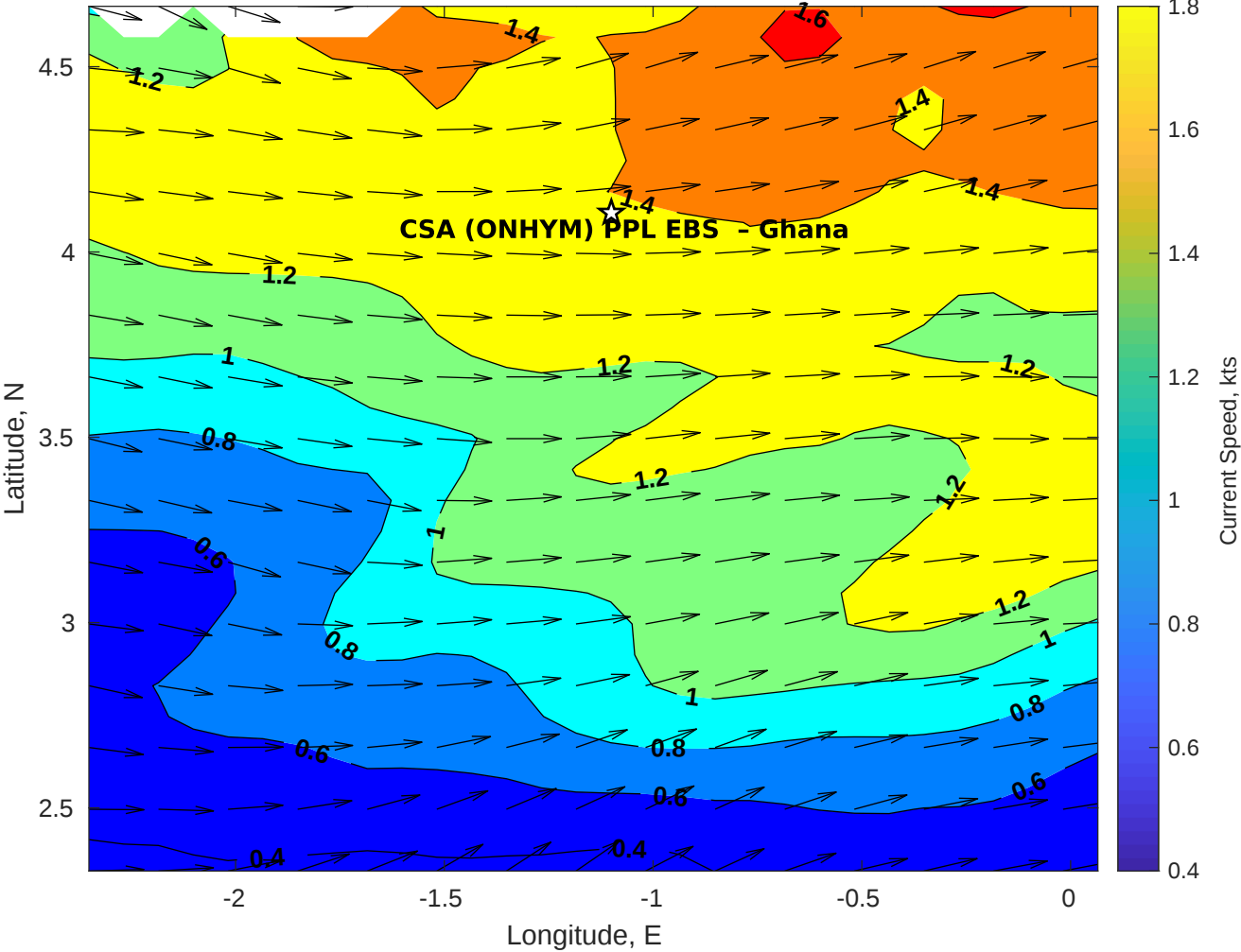
Surface Currents for CSA (ONHYM) PPL EBS - Ghana at 15-Aug-2025 00:00:00
