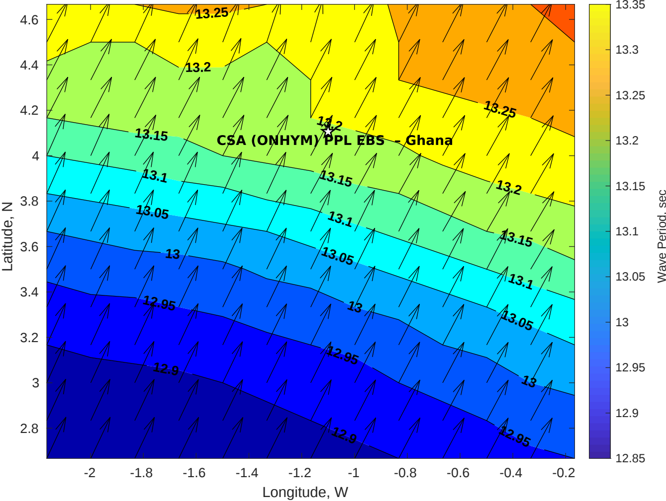
Wave Period (sec) for CSA (ONHYM) PPL EBS - Ghana at 16-Aug-2025 09:00:00
