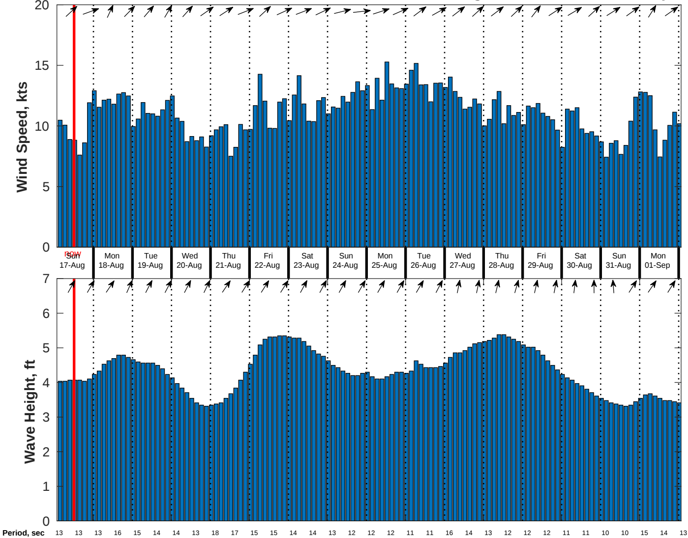
Wind & Wave Forecast for CSA (ONHYM) PPL EBS - Ghana from 16-Aug-2025 02:00:00 to 01-Sep-2025 02:00:00
