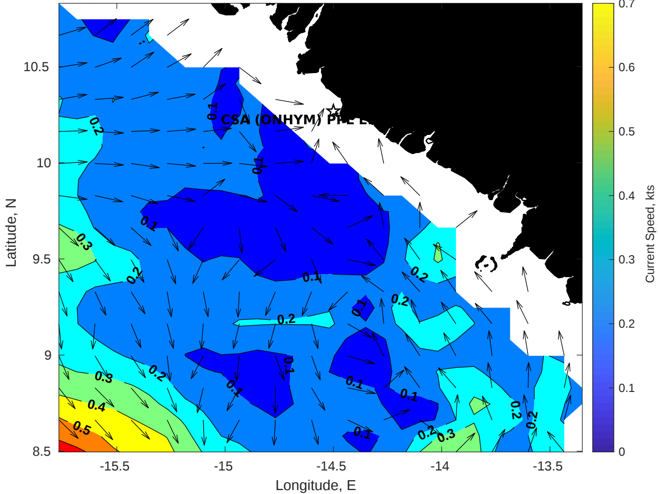
Surface Currents for CSA (ONHYM) PPL EBS - Guinea at 15-Aug-2025 00:00:00
