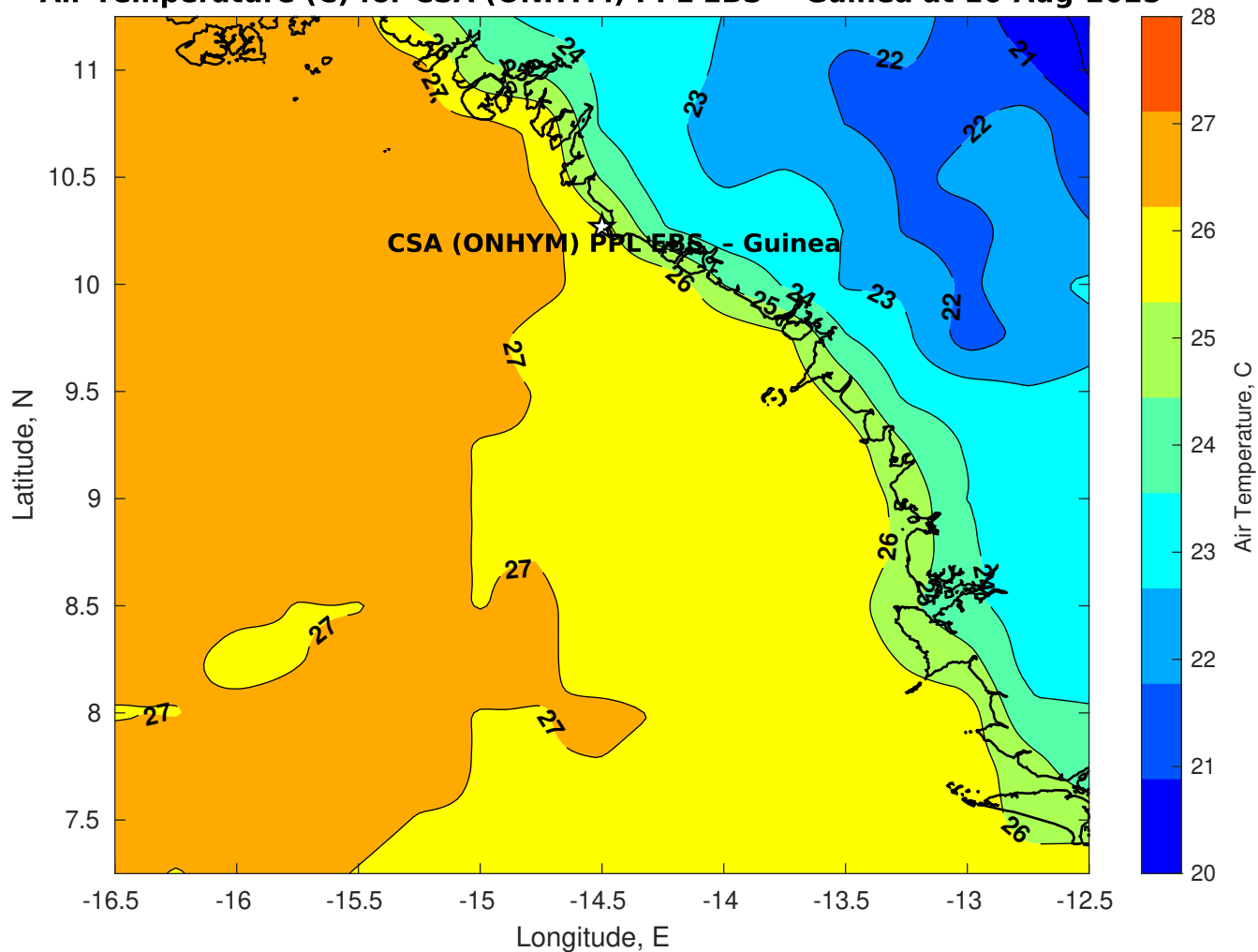
Air Temperature (C) for CSA (ONHYM) PPL EBS - Guinea at 16-Aug-2025
