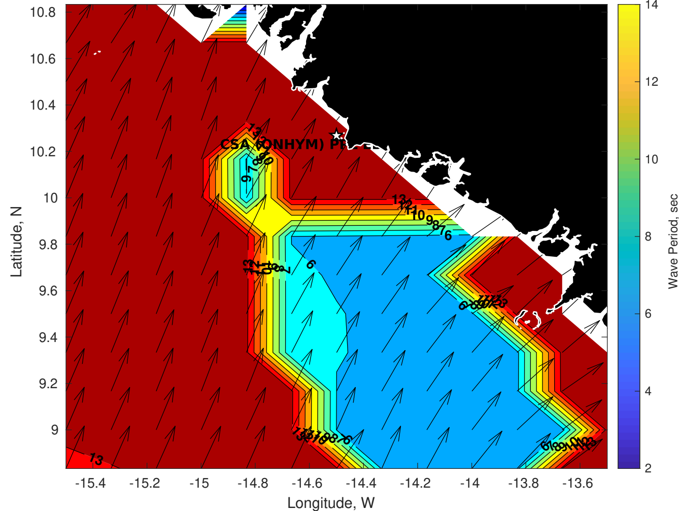
Wave Period (sec) for CSA (ONHYM) PPL EBS - Guinea at 16-Aug-2025 09:00:00
