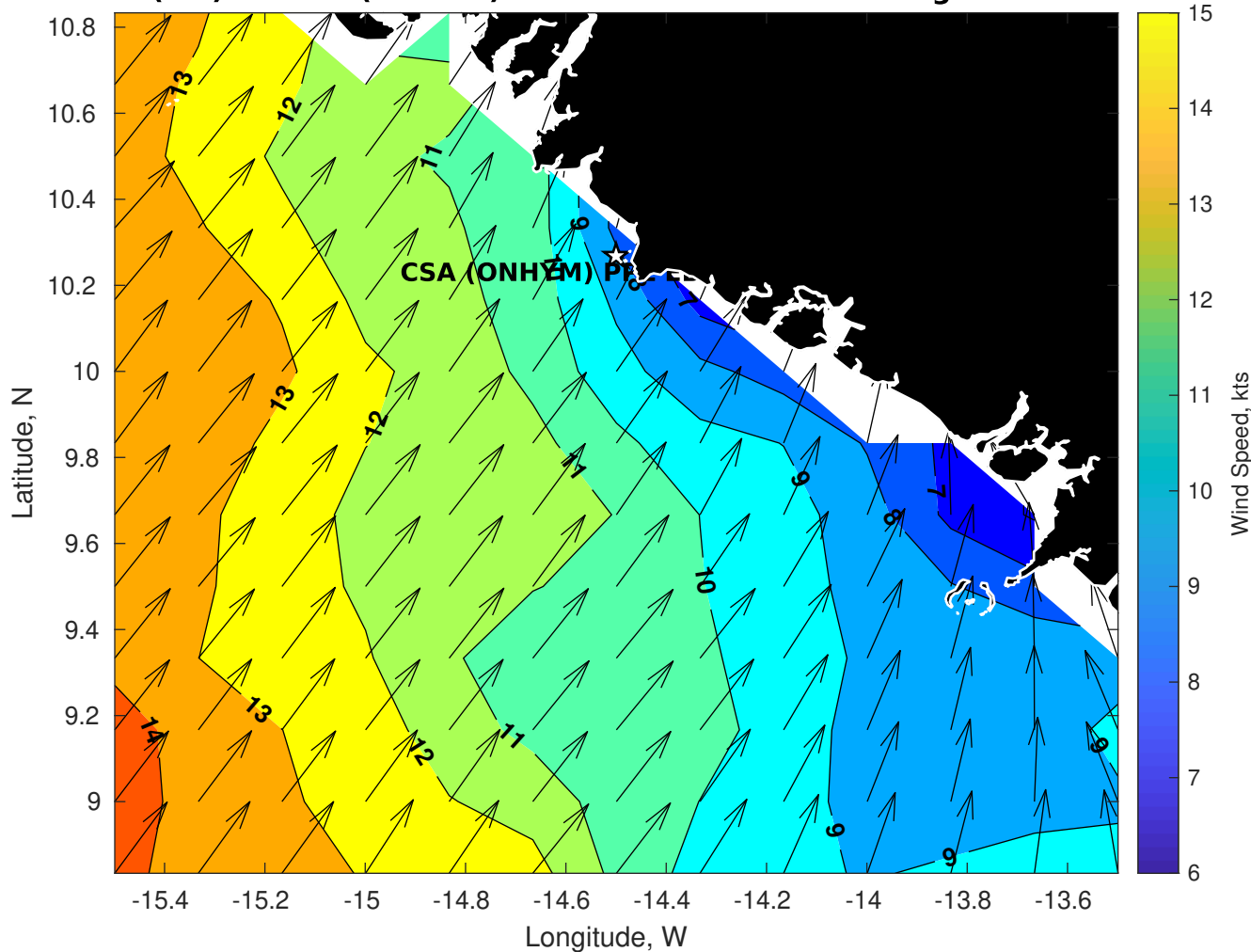
Winds (kts) for CSA (ONHYM) PPL EBS - Guinea at 16-Aug-2025 09:00:00
