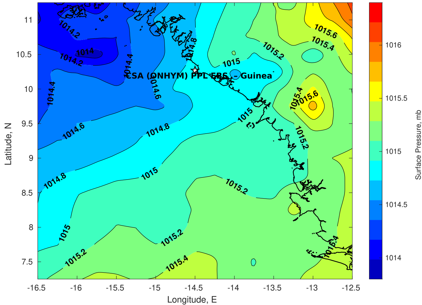
Surface Pressure (mb) for CSA (ONHYM) PPL EBS - Guinea at 18-Aug-2025 00:00:00
