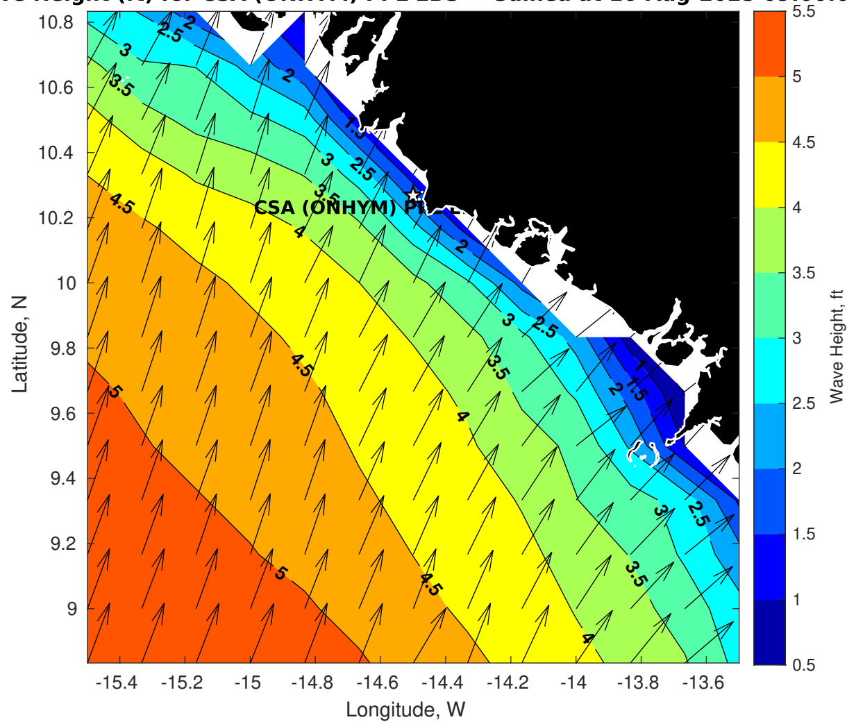
Wave Height (ft) for CSA (ONHYM) PPL EBS - Guinea at 16-Aug-2025 09:00:00
