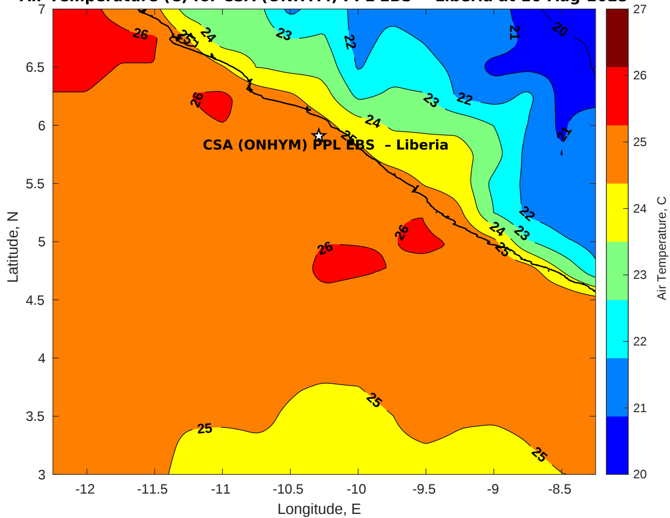
Air Temperature (C) for CSA (ONHYM) PPL EBS - Liberia at 16-Aug-2025
