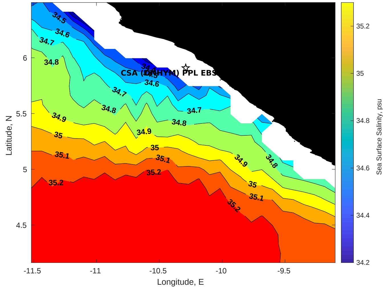
Surface Salinity for CSA (ONHYM) PPL EBS - Liberia at 15-Aug-2025 00:00:00
