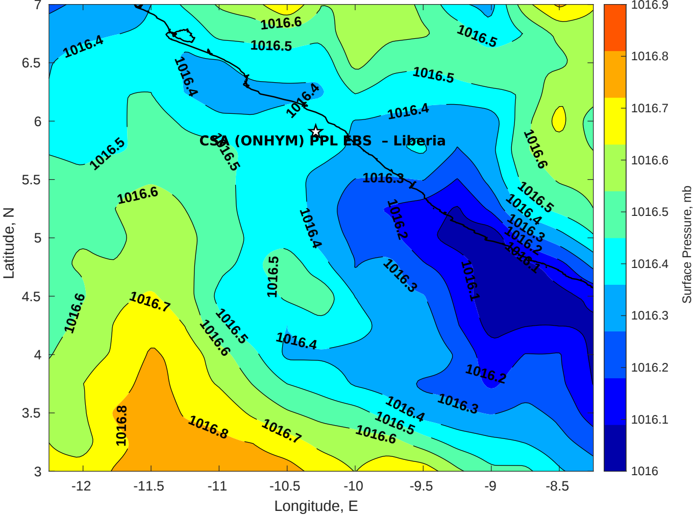
Surface Pressure (mb) for CSA (ONHYM) PPL EBS - Liberia at 16-Aug-2025 00:00:00
