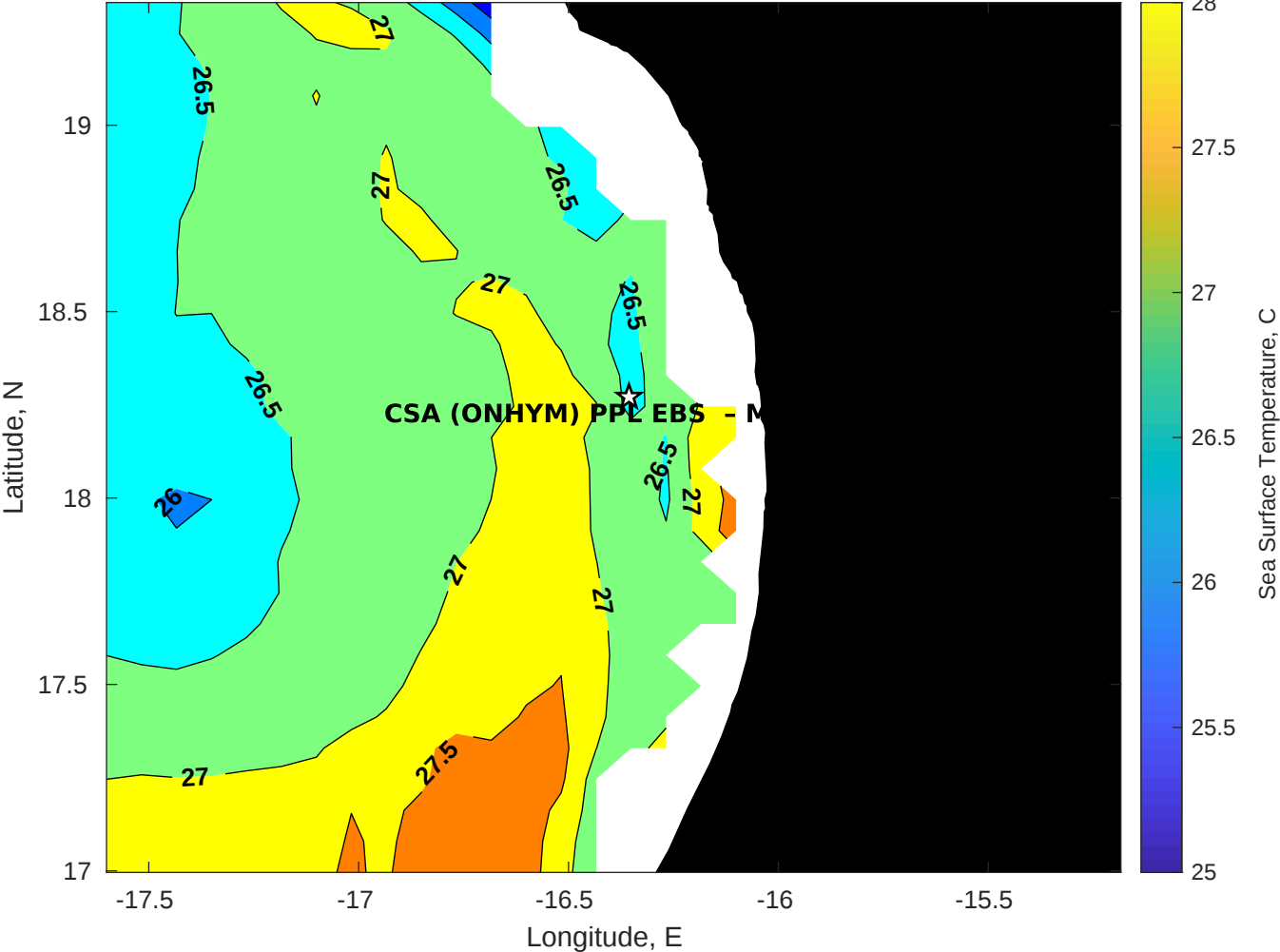
SST for CSA (ONHYM) PPL EBS - Mauritania at 15-Aug-2025 00:00:00
