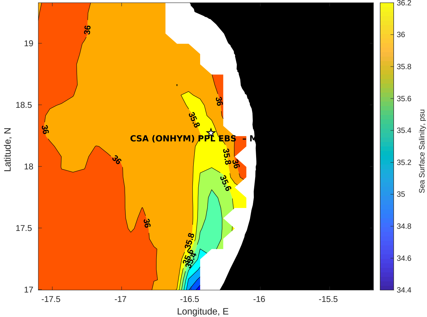
Surface Salinity for CSA (ONHYM) PPL EBS - Mauritania at 15-Aug-2025 00:00:00
