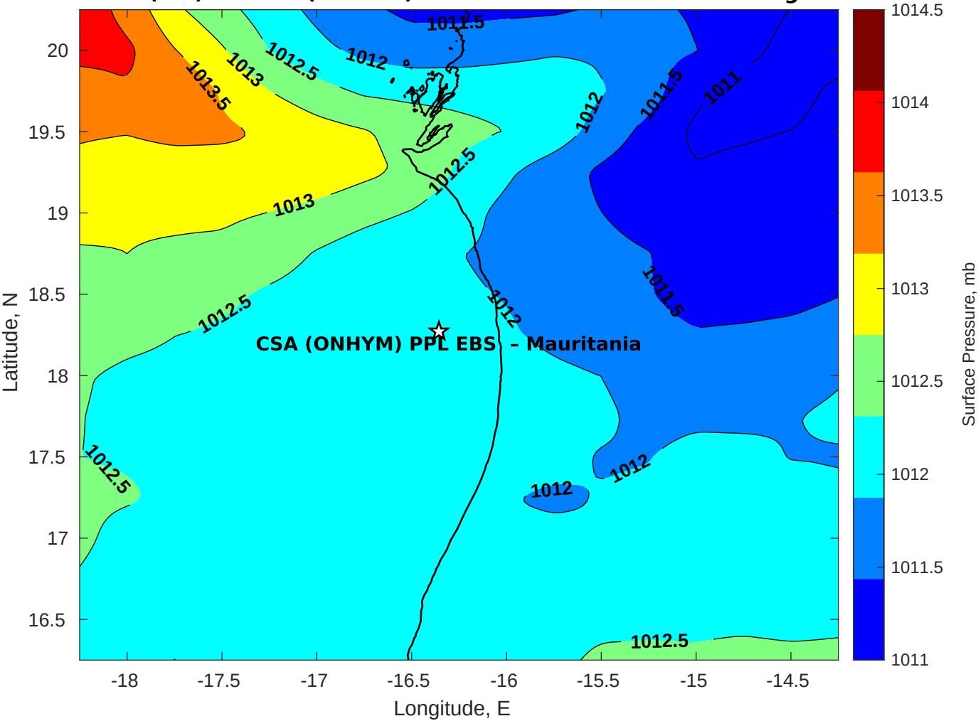
Surface Pressure (mb) for CSA (ONHYM) PPL EBS - Mauritania at 17-Aug-2025 00:00:00
