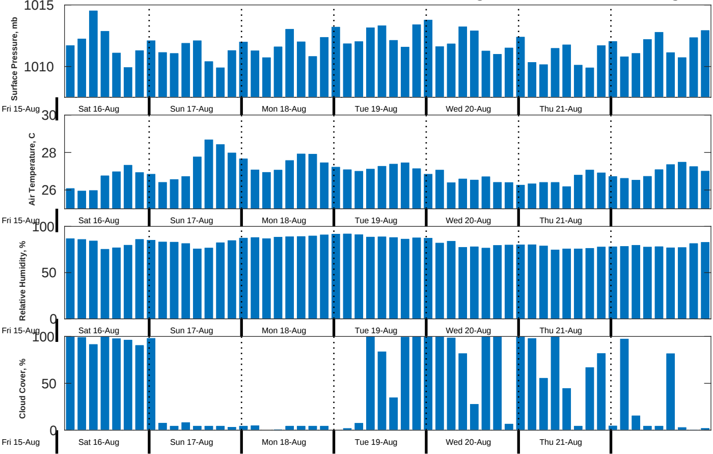
Met Forecast for CSA (ONHYM) PPL EBS - Mauritania from 16-Aug-2025 00:00:00 to 23-Aug-2025 00:00:00
