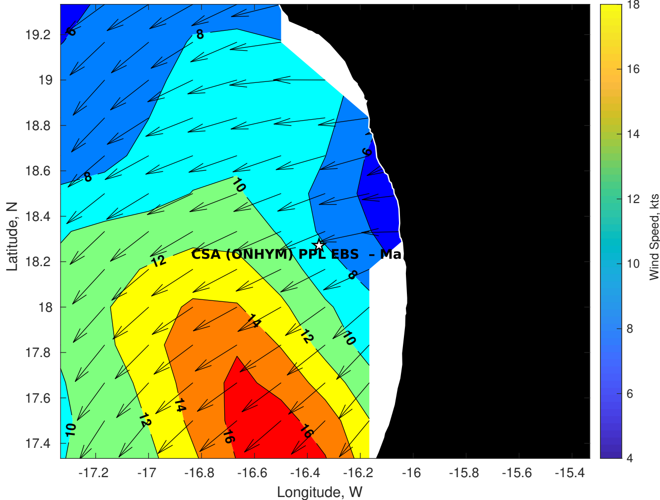
Winds (kts) for CSA (ONHYM) PPL EBS - Mauritania at 16-Aug-2025 09:00:00
