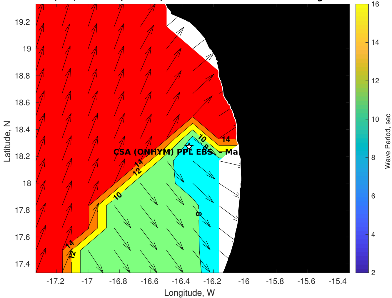
Wave Period (sec) for CSA (ONHYM) PPL EBS - Mauritania at 16-Aug-2025 09:00:00
