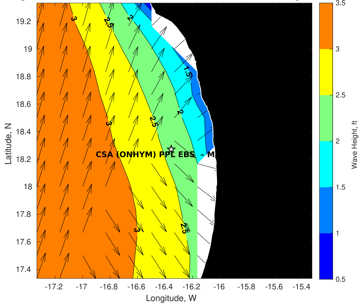
Wave Height (ft) for CSA (ONHYM) PPL EBS - Mauritania at 16-Aug-2025 09:00:00
