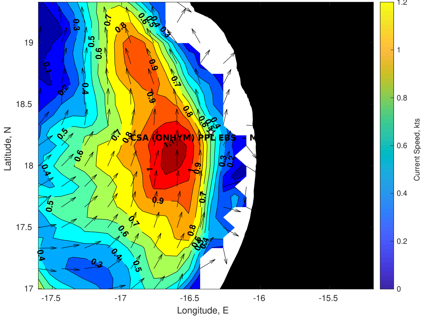
Surface Currents for CSA (ONHYM) PPL EBS - Mauritania at 15-Aug-2025 00:00:00
