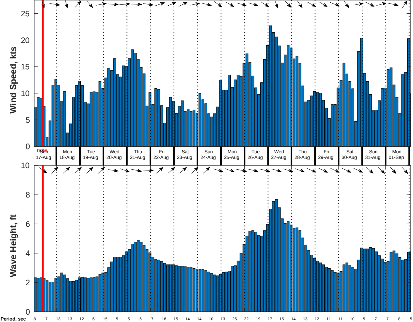
Wind & Wave Forecast for CSA (ONHYM) PPL EBS - Mauritania from 16-Aug-2025 01:00:00 to 01-Sep-2025 01:00:00
