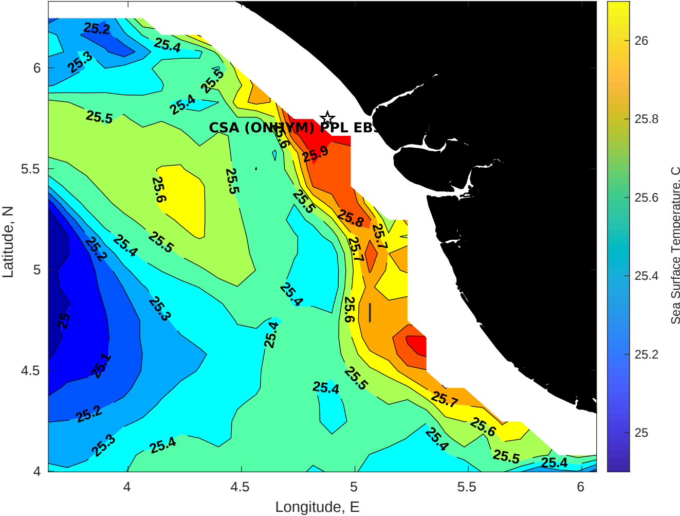
SST for CSA (ONHYM) PPL EBS - Nigeria at 15-Aug-2025 00:00:00
