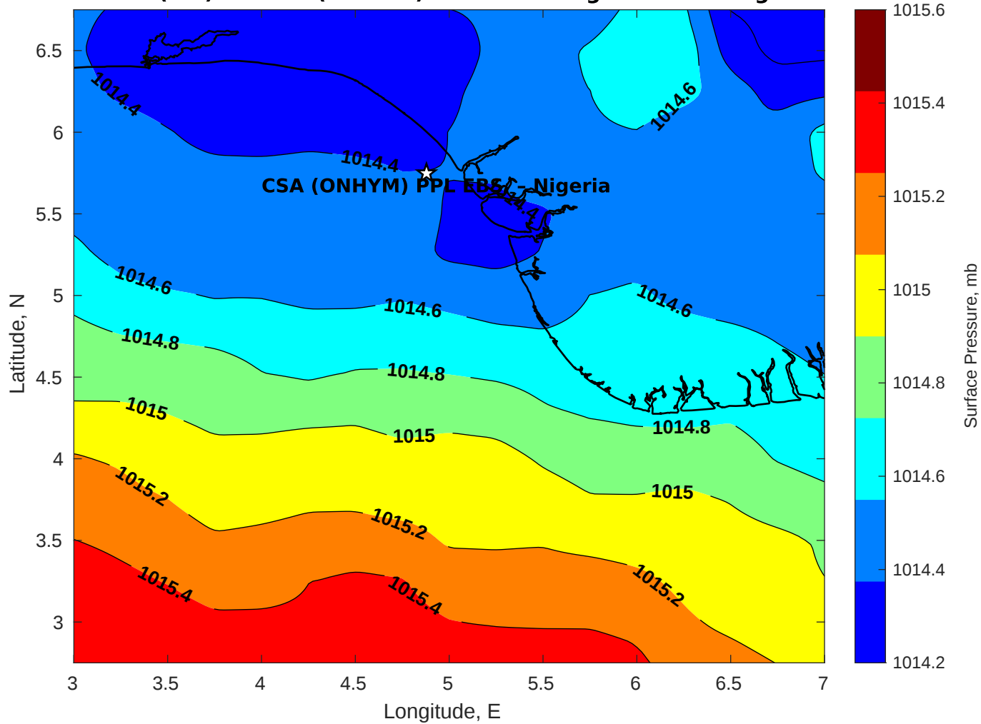
Surface Pressure (mb) for CSA (ONHYM) PPL EBS - Nigeria at 18-Aug-2025 00:00:00
