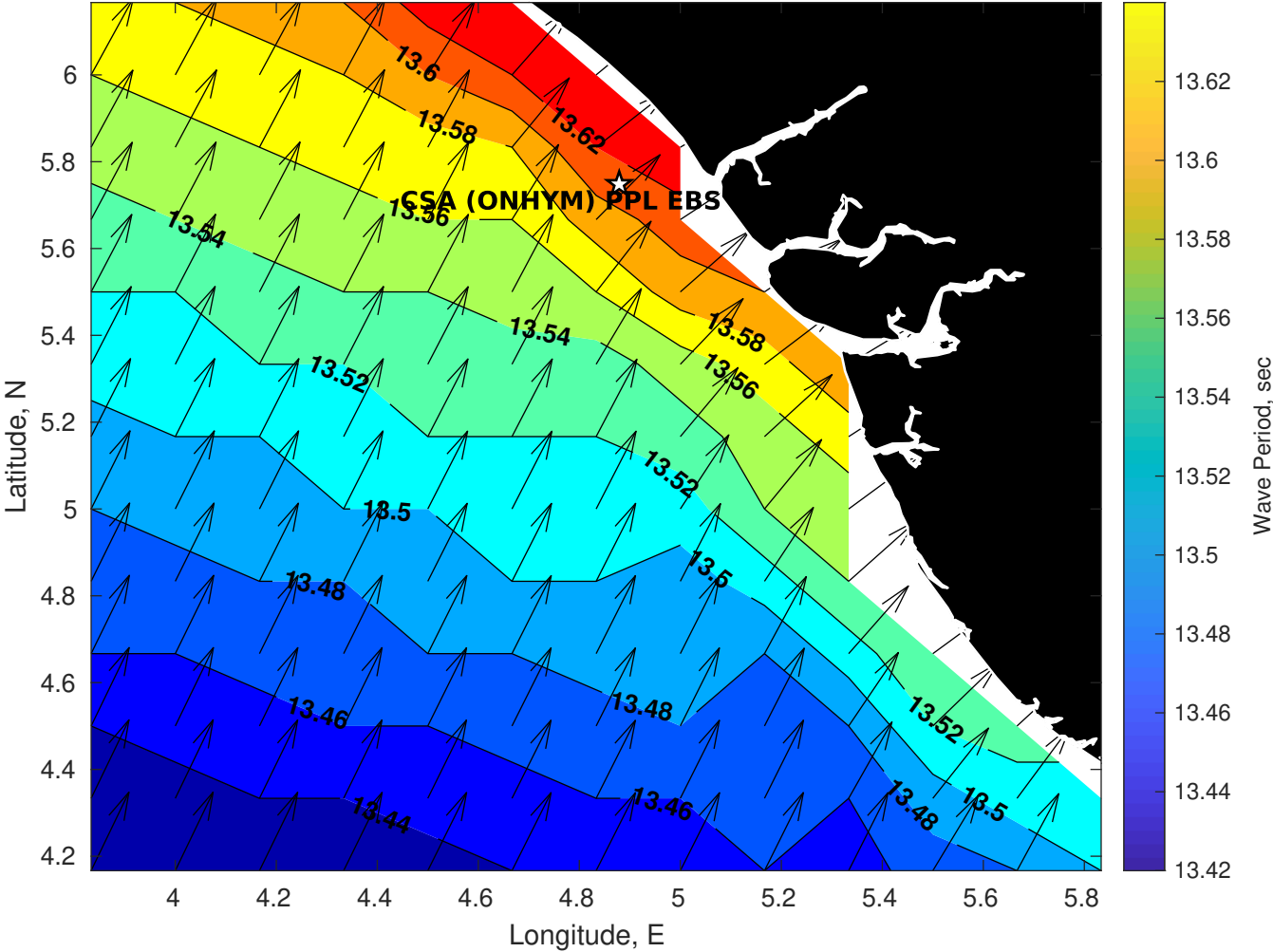
Wave Period (sec) for CSA (ONHYM) PPL EBS - Nigeria at 16-Aug-2025 09:00:00
