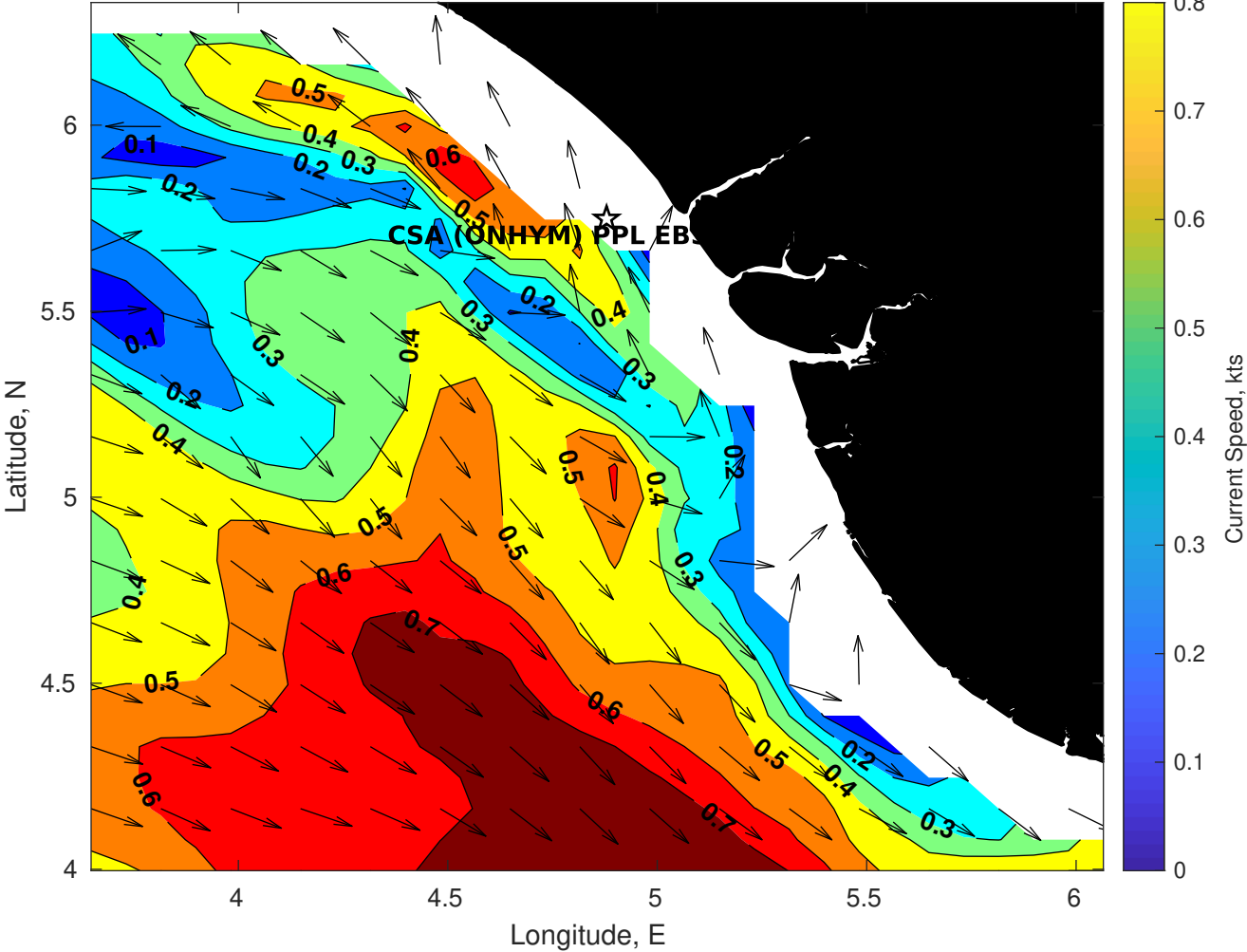
Surface Currents for CSA (ONHYM) PPL EBS - Nigeria at 15-Aug-2025 00:00:00
