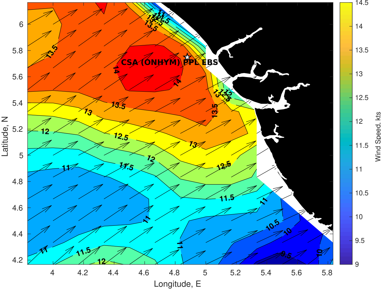
Winds (kts) for CSA (ONHYM) PPL EBS - Nigeria at 16-Aug-2025 09:00:00
