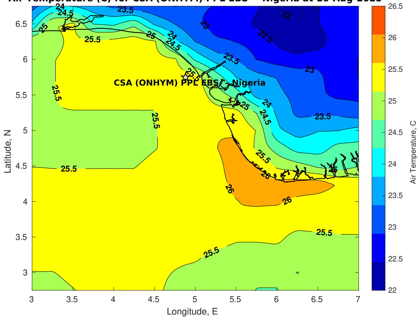
Air Temperature (C) for CSA (ONHYM) PPL EBS - Nigeria at 16-Aug-2025
