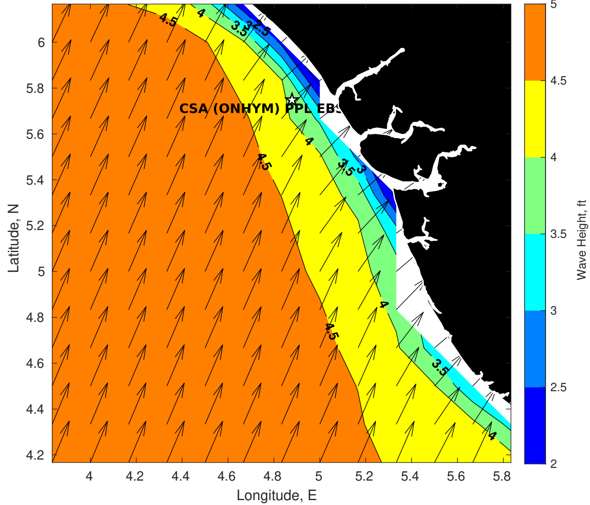
Wave Height (ft) for CSA (ONHYM) PPL EBS - Nigeria at 16-Aug-2025 09:00:00
