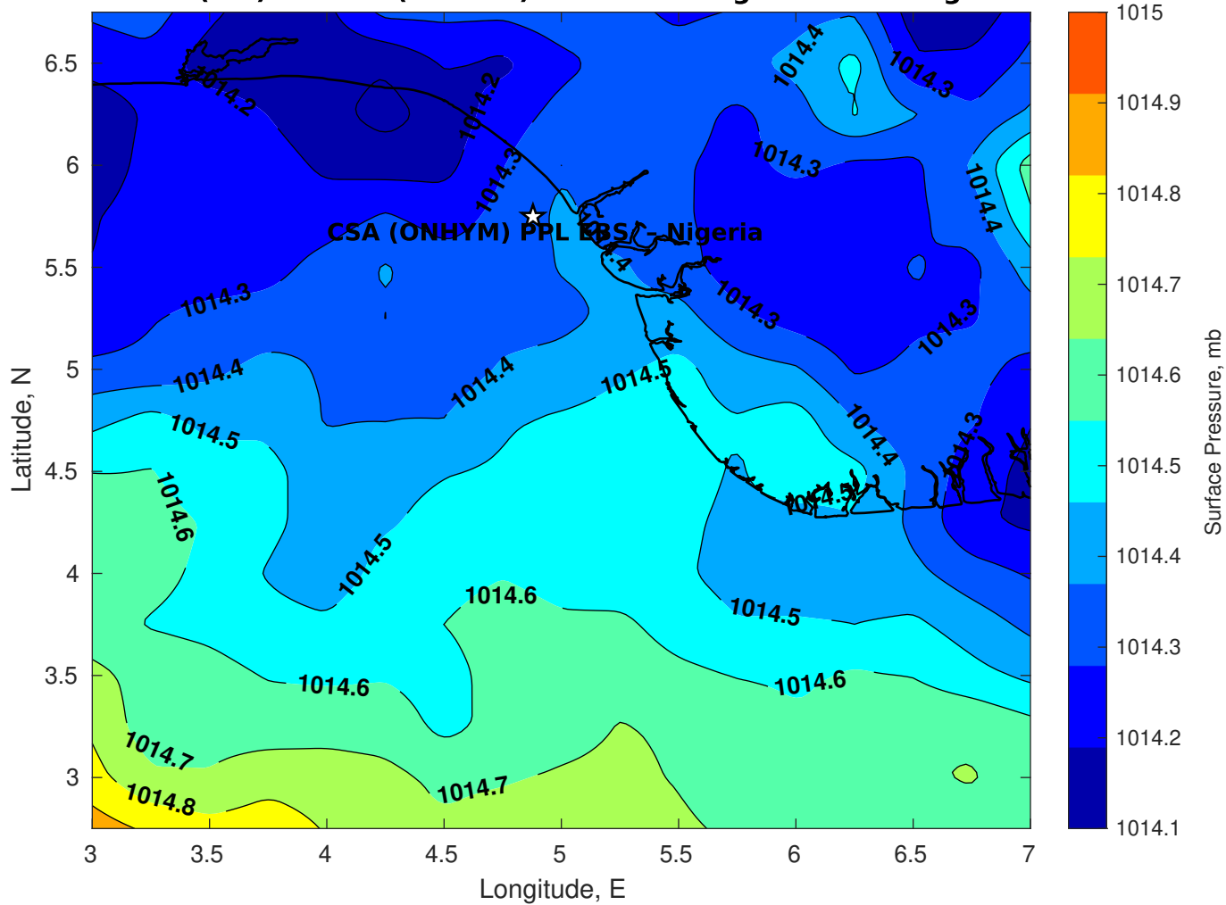
Surface Pressure (mb) for CSA (ONHYM) PPL EBS - Nigeria at 17-Aug-2025 00:00:00
