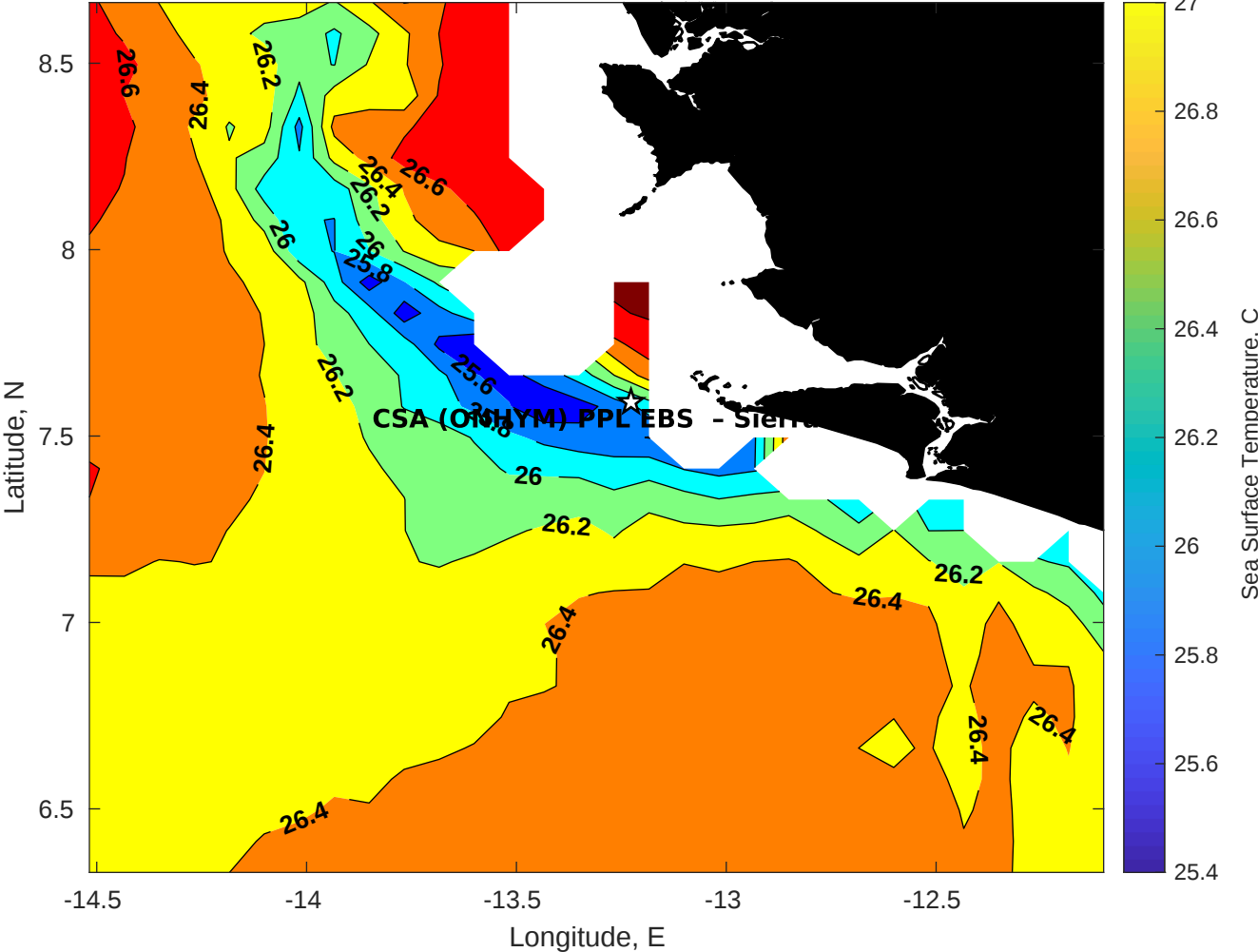
SST for CSA (ONHYM) PPL EBS - Sierra Leone at 15-Aug-2025 00:00:00
