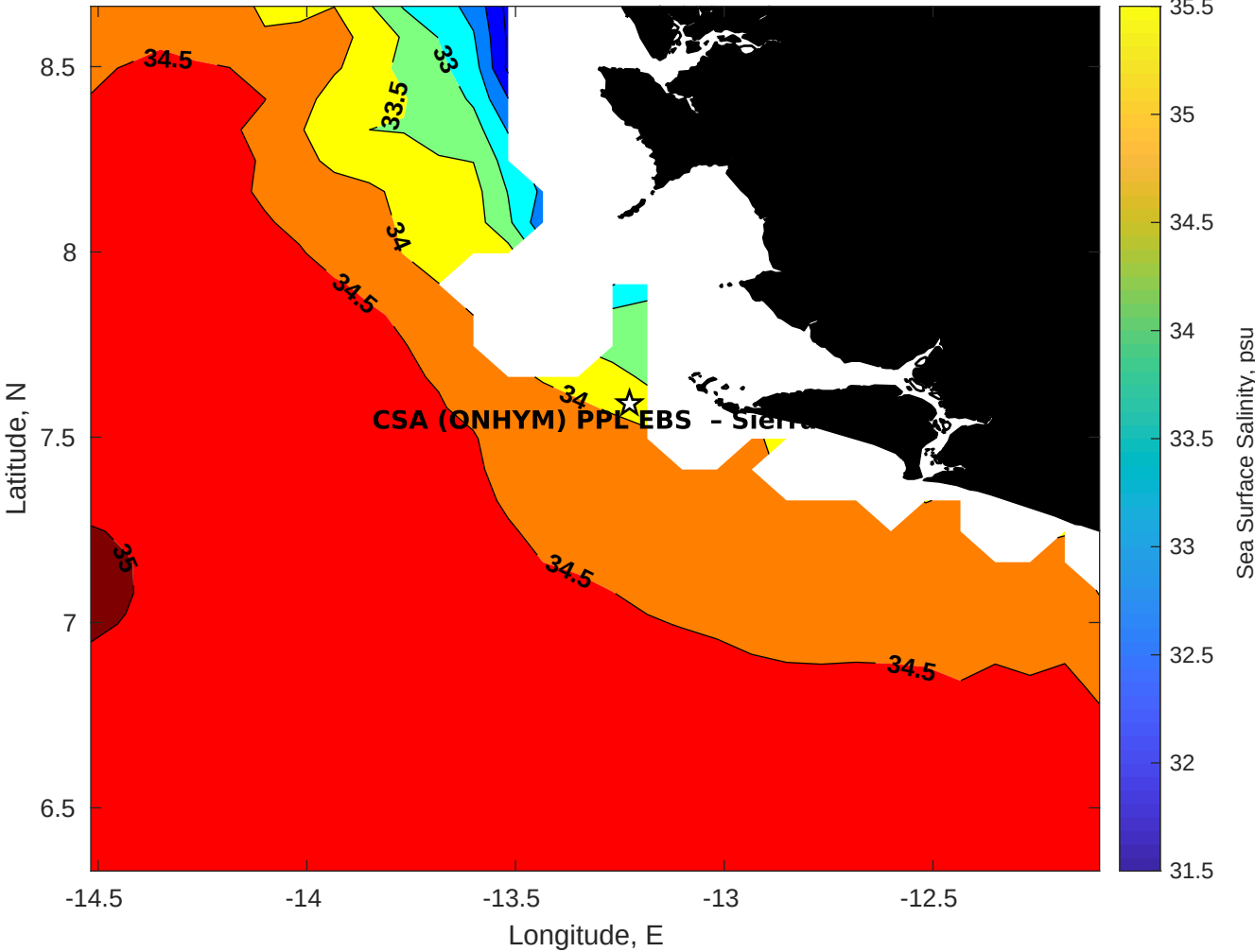
Surface Salinity for CSA (ONHYM) PPL EBS - Sierra Leone at 15-Aug-2025 00:00:00
