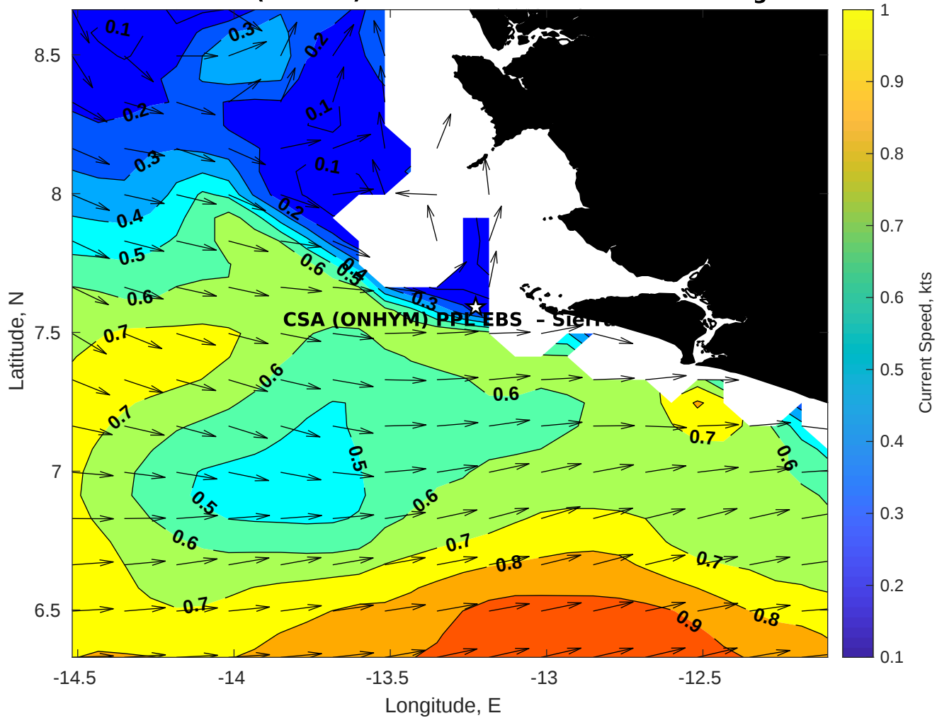
Surface Currents for CSA (ONHYM) PPL EBS - Sierra Leone at 15-Aug-2025 00:00:00
