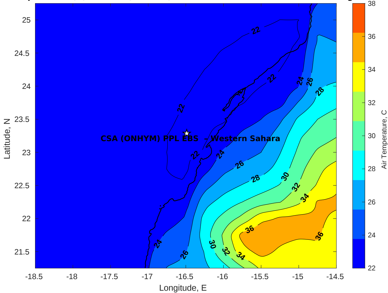
Air Temperature (C) for CSA (ONHYM) PPL EBS - Western Sahara at 16-Aug-2025
