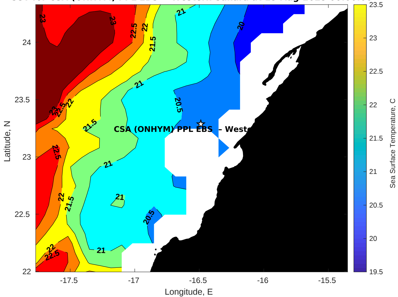
SST for CSA (ONHYM) PPL EBS - Western Sahara at 15-Aug-2025 00:00:00
