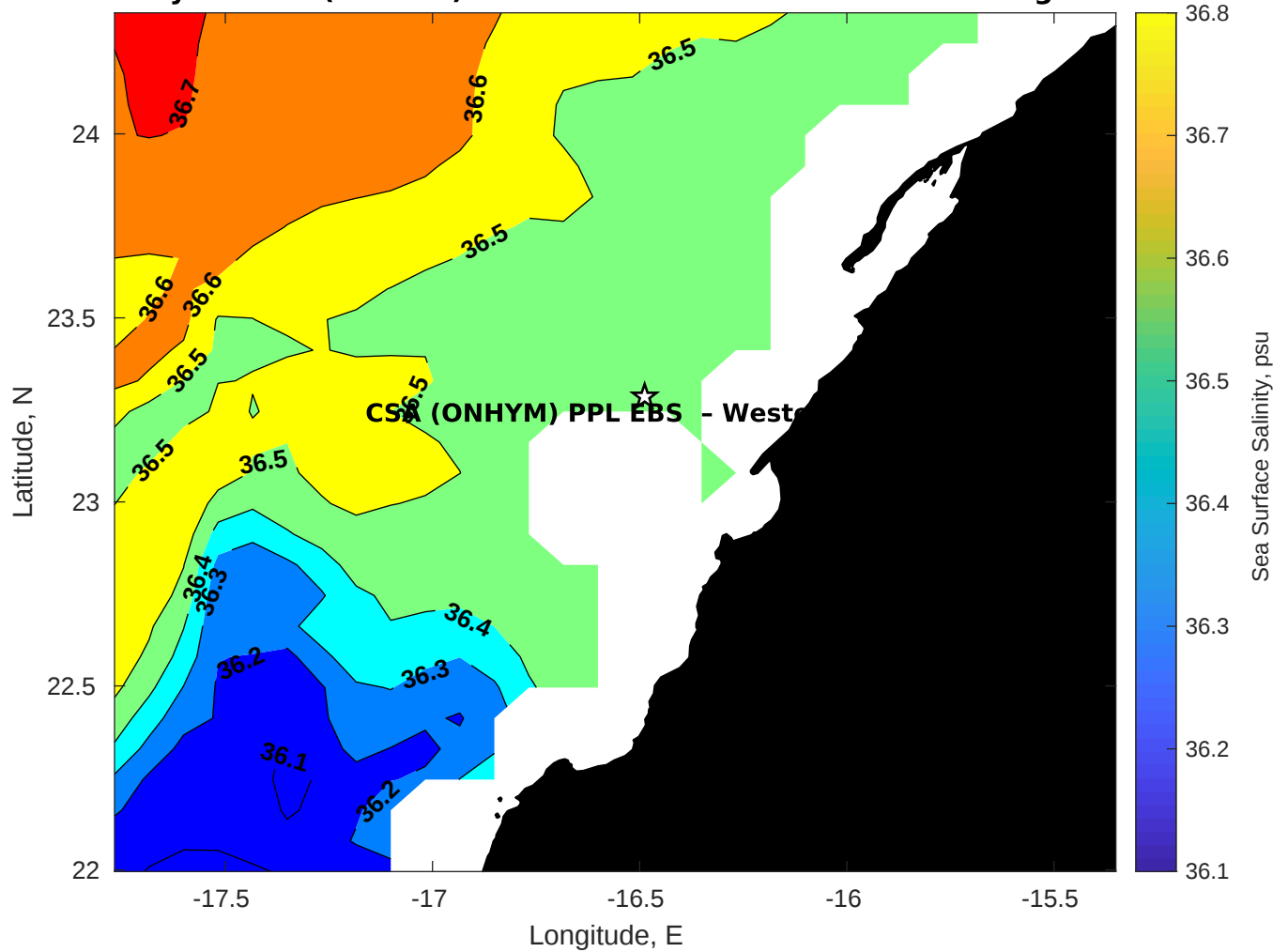
Surface Salinity for CSA (ONHYM) PPL EBS - Western Sahara at 15-Aug-2025 00:00:00
