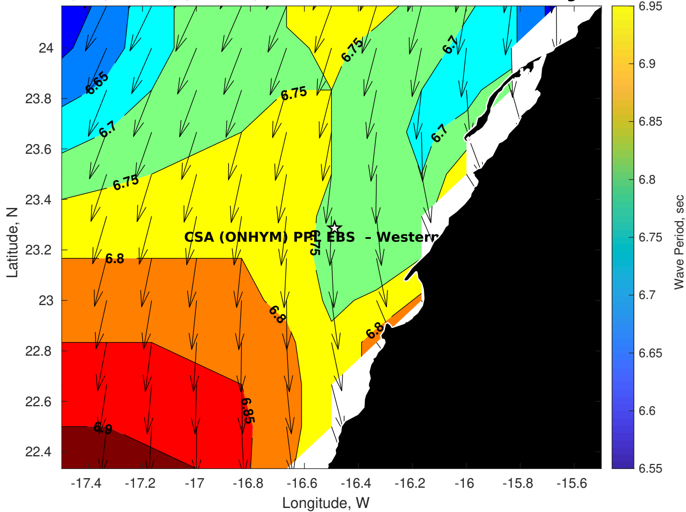
Wave Period (sec) for CSA (ONHYM) PPL EBS - Western Sahara at 16-Aug-2025 09:00:00
