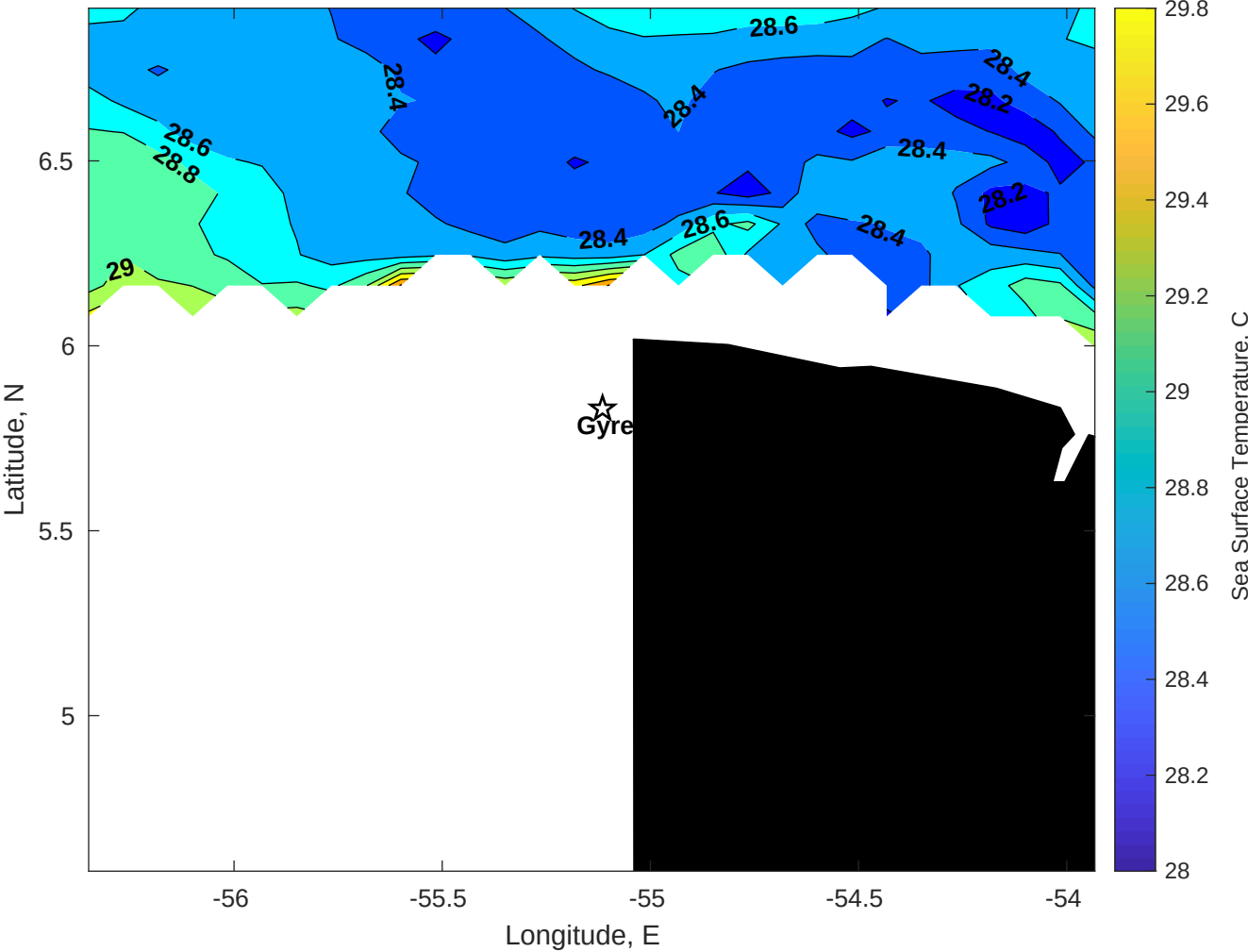
SST for Gyre at 15-Aug-2025 00:00:00
